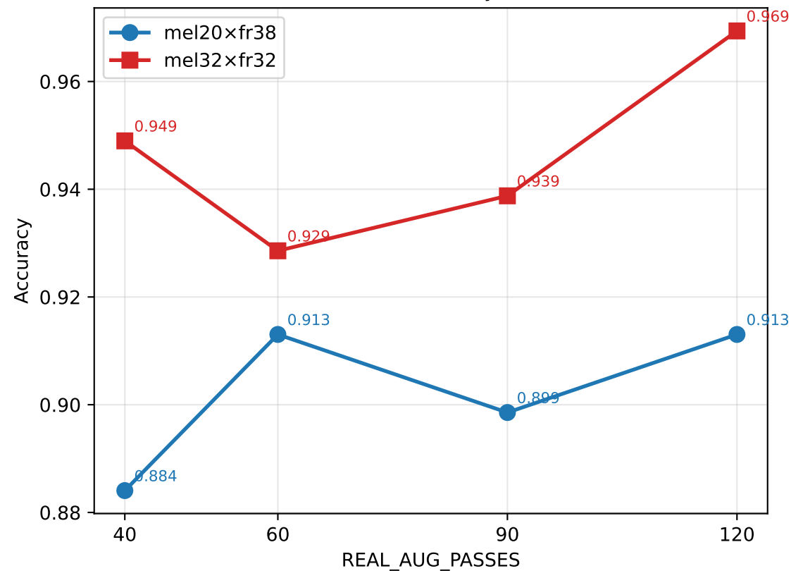
Val accuracy
