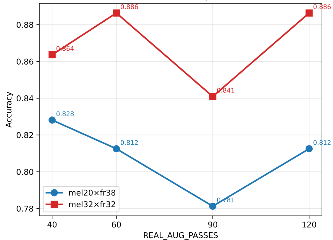
Test accuracy
