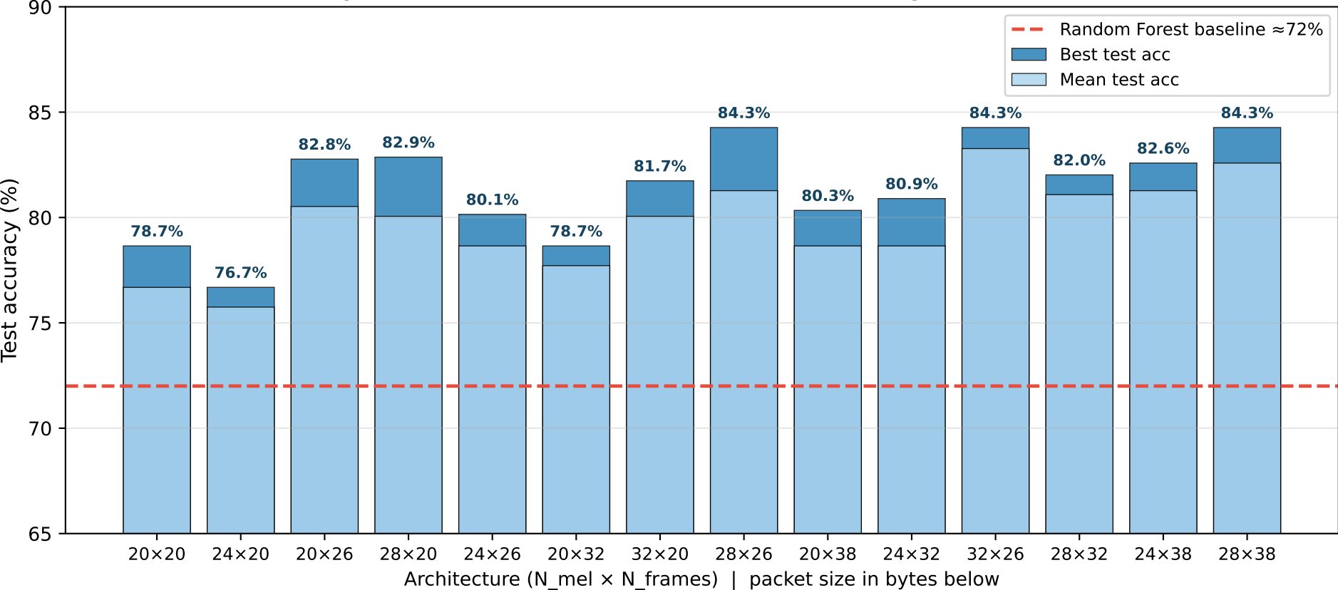
Accuracy vs. Architecture — Best and Mean over Augmentation Profiles
