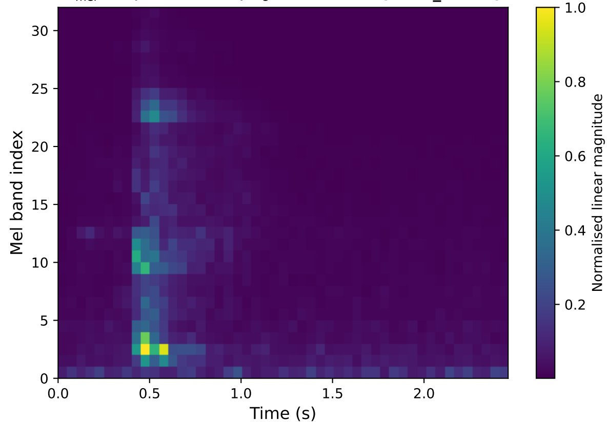
Mel spectrogram — Gunshot N_{mel}=32 , HOP=512, f_s=10200 Hz (mcu_linear)
