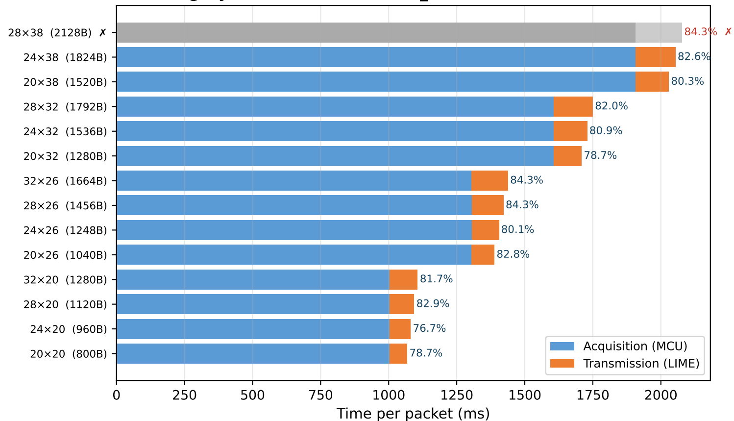
Time breakdown: acquisition vs. LIME transmission (grey / \times = PASSTHROUGH_LEN > 65535, infeasible)
