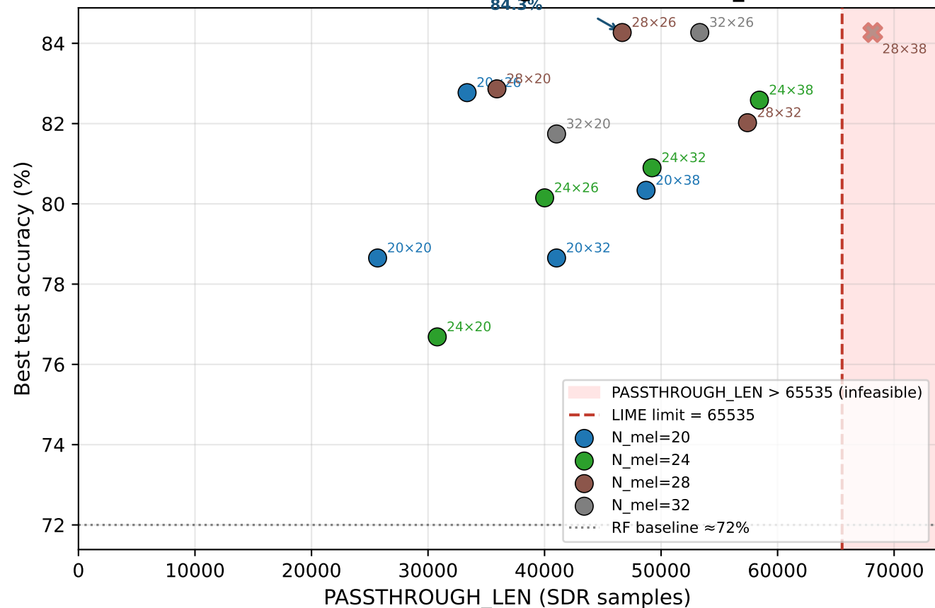
Accuracy vs. LIME constraint ( \times = architectures exceeding PASSTHROUGH_LEN limit)
