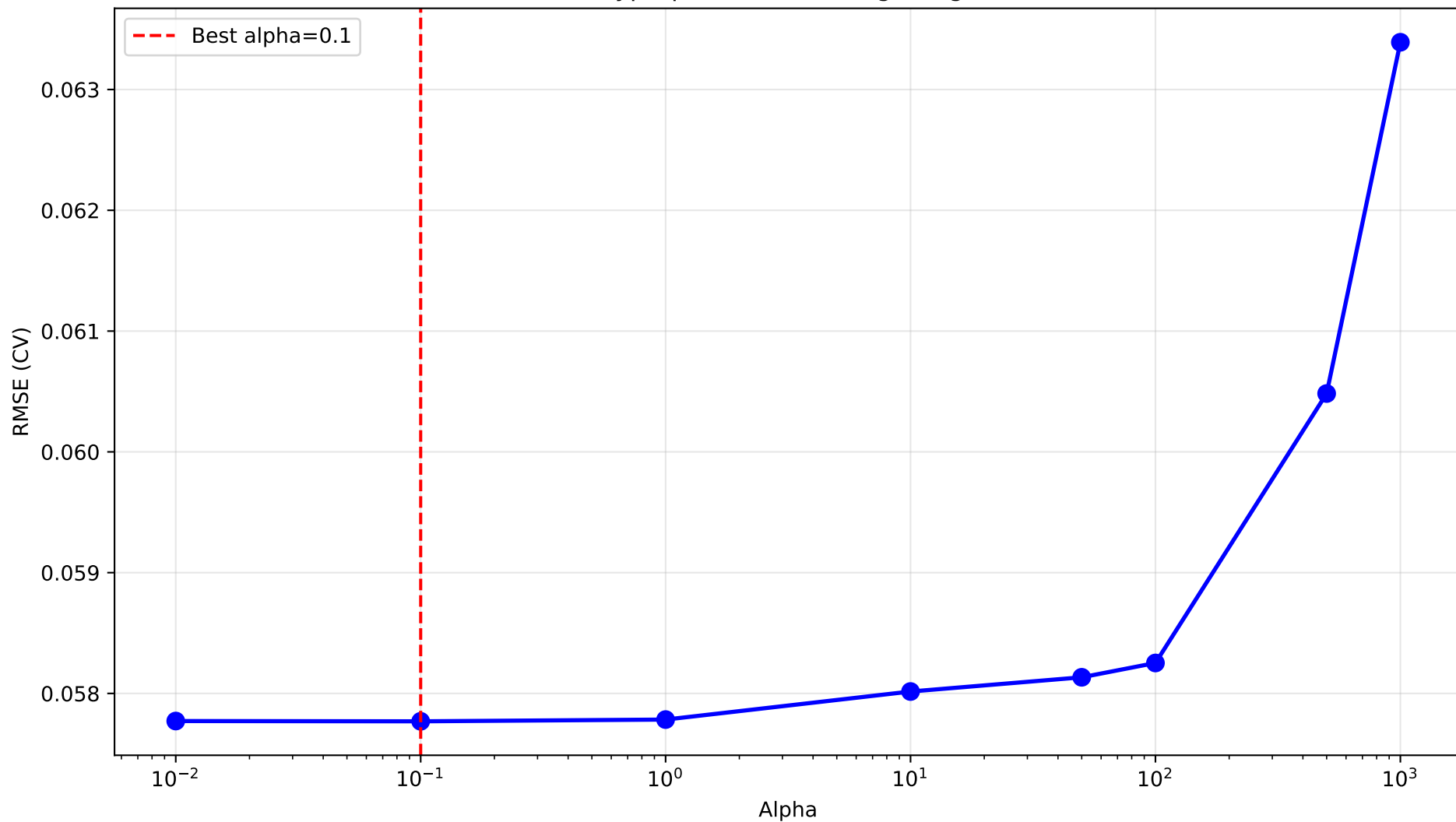
Hyperparameter Tuning: Ridge
