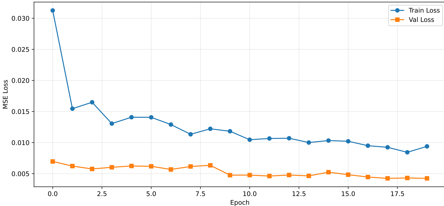
CNN Training Progress
