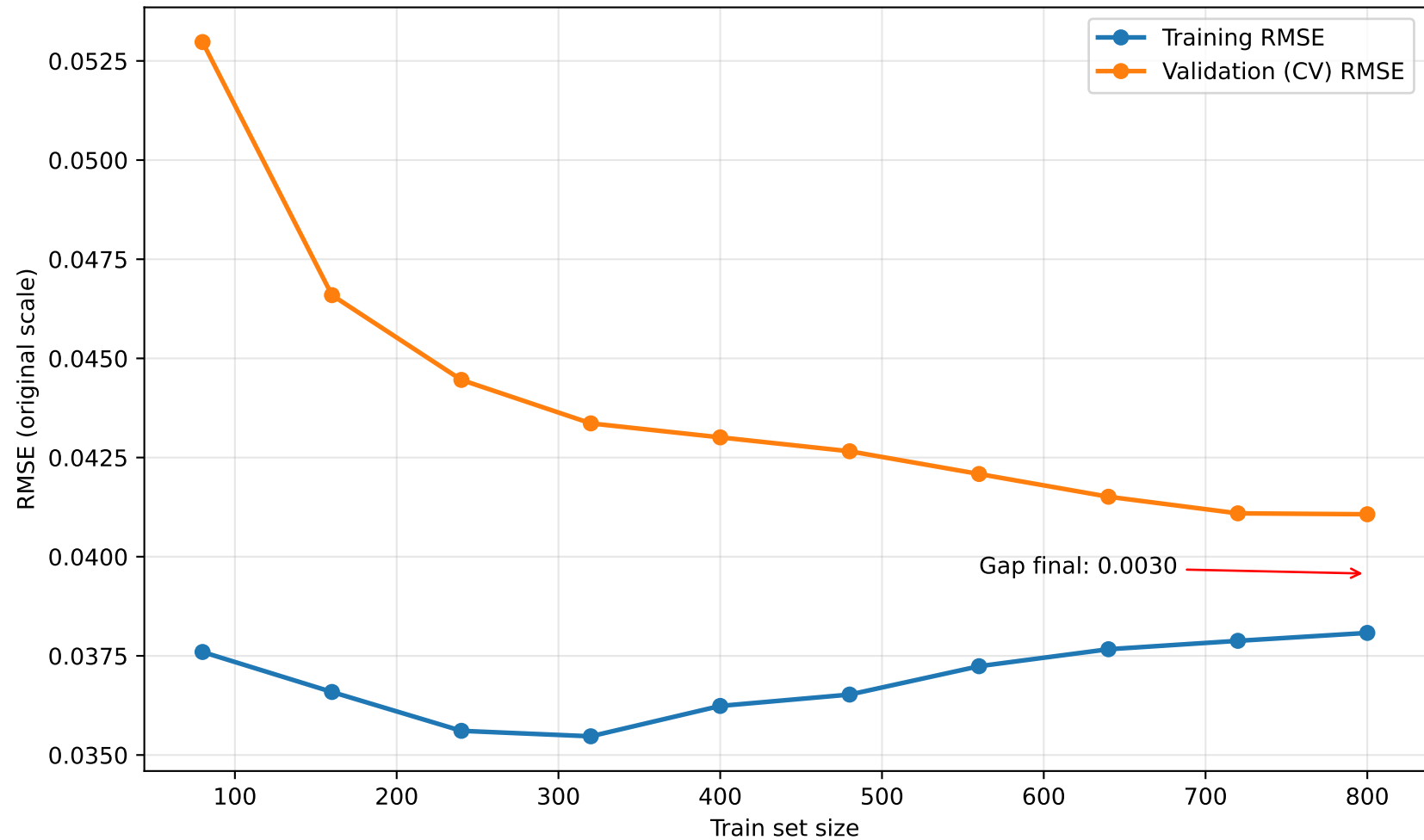
Learning Curve (11 features)
