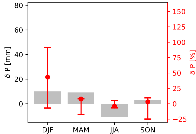
CESM2-WACCM-FV2
