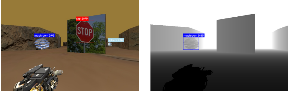
Figure 4: Artefact detections using RGB (left) and depth (right). Both models detect the mushroom; the stop sign and distant sphere are detected only in the RGB image.
