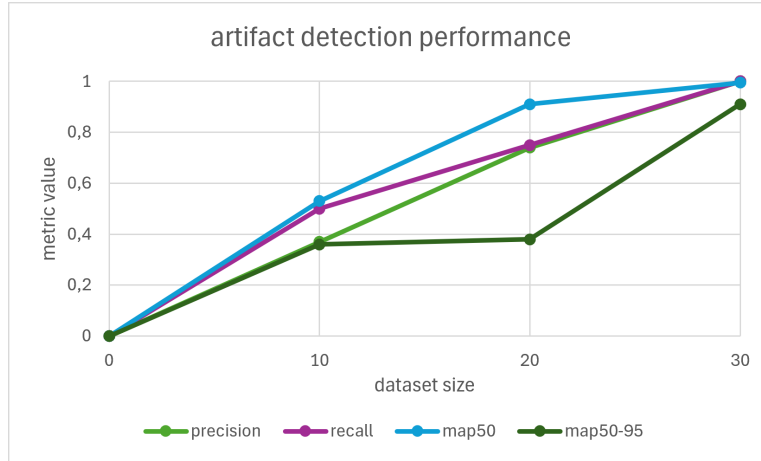
Figure 1: Detection performance for the alien artefact with increasing dataset size. Precision and recall reach 1.0 on the test split at 30 images.
