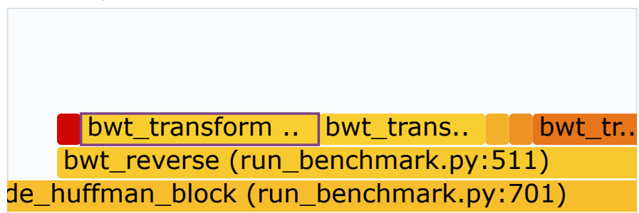
Figure 3: Full optimized Python profile, before native offload. Inverse BWT and its index-table construction remain visible. Matcher work was inlined, so its old function frame disappears without implying that Huffman decoding is free.
