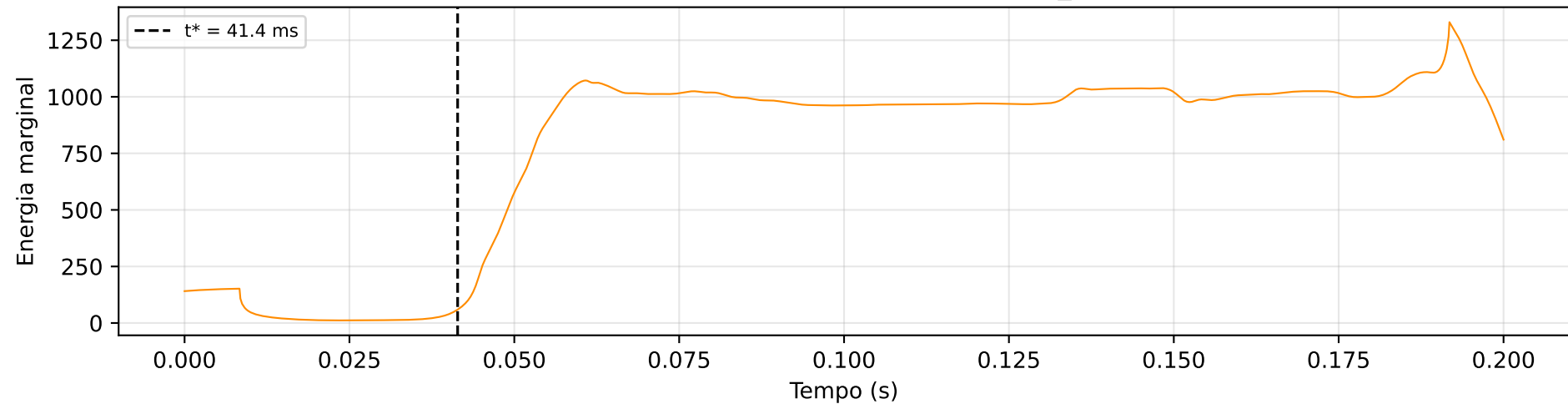
Energia marginal das IMFs — sinal_9
