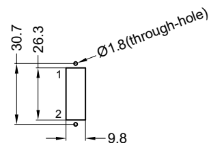
Detail A , 2:1 (Adapter installation size)
