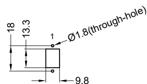
Detail A , 2:1 (Adapter installation size)
