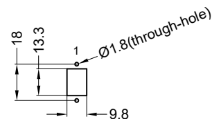
Detail A , 2:1 (Adapter installation size)
