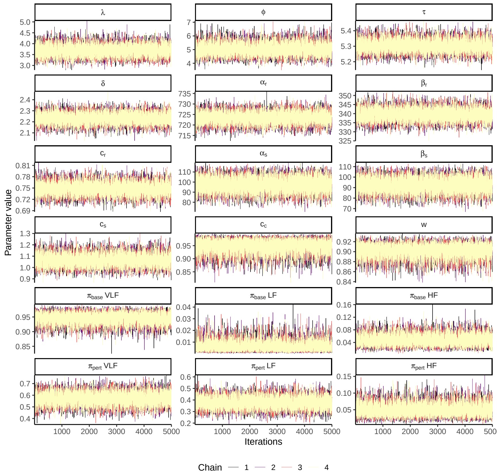
Stationary distribution of model parameters
