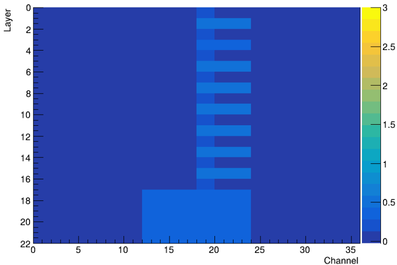
Beam profile for 20 GeV tagged MUON in a MUON beam
