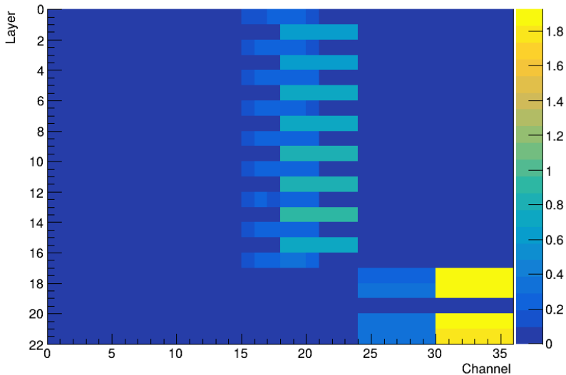
Beam profile for 160 GeV tagged LATE_HADRON in a MUON beam
