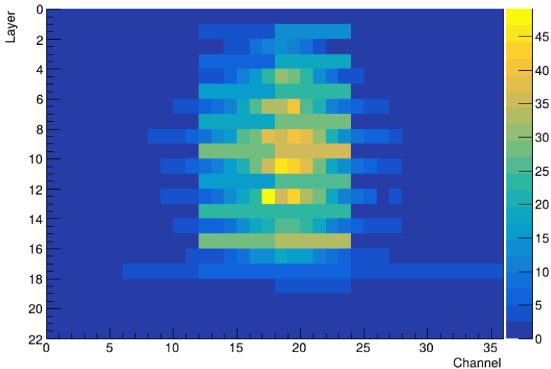
Beam profile for 300 GeV tagged ELECTRON in a MUON beam
