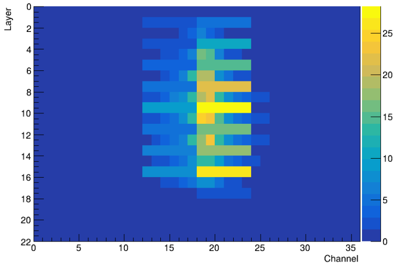
Beam profile for 140 GeV tagged ELECTRON in a MUON beam
