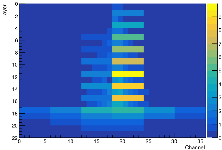
Beam profile for 30 GeV tagged EARLY_HADRON in a MUON beam
