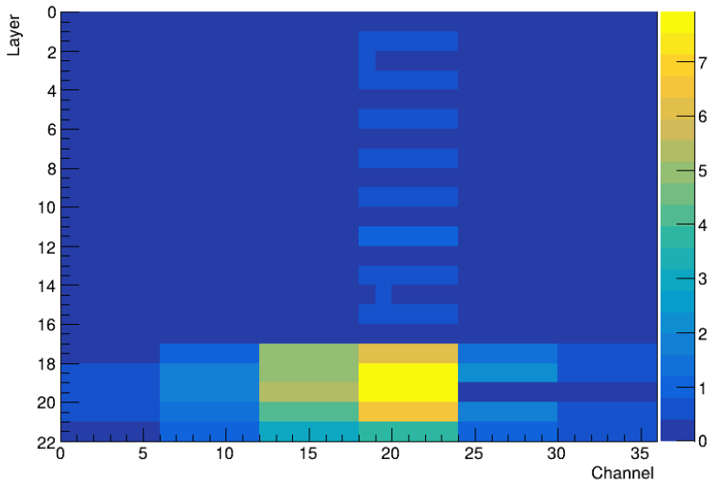
Beam profile for 100 GeV tagged LATE_HADRON in a MUON beam
