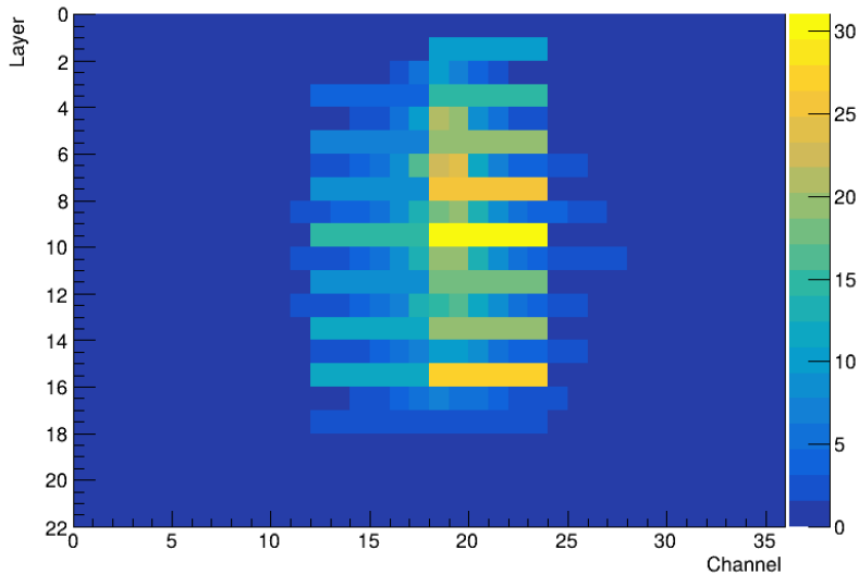
Beam profile for 100 GeV tagged ELECTRON in a MUON beam
