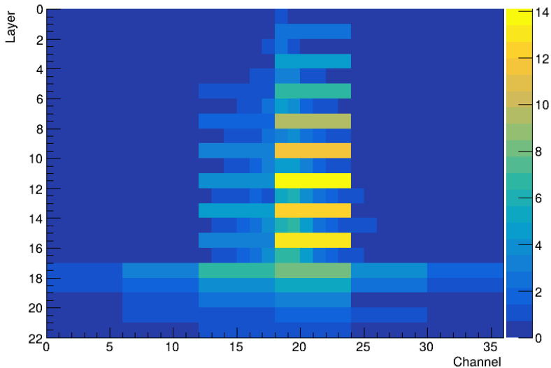
Beam profile for 50 GeV tagged EARLY_HADRON in a MUON beam
