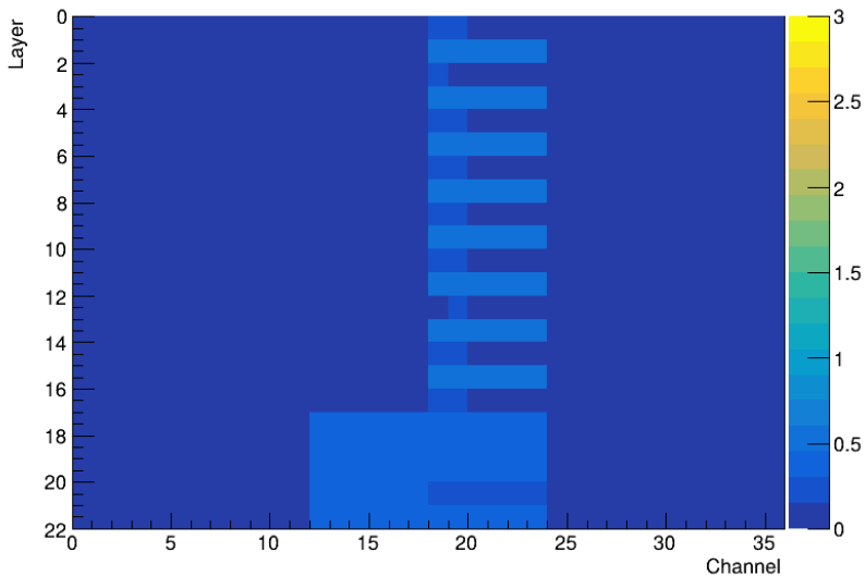
Beam profile for 15 GeV tagged MUON in a MUON beam
