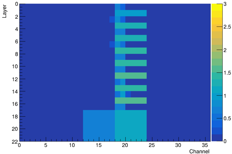
Beam profile for 180 GeV tagged MUON in a MUON beam
