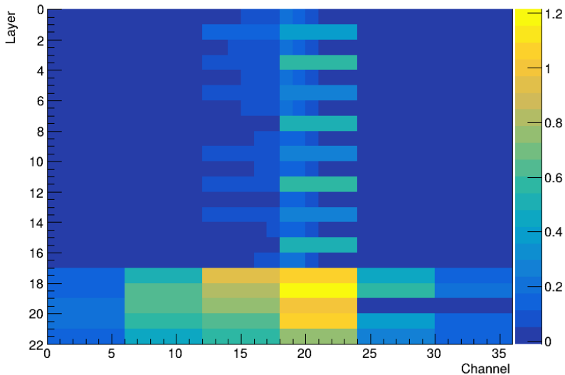
Beam profile for 140 GeV tagged LATE_HADRON in a MUON beam
