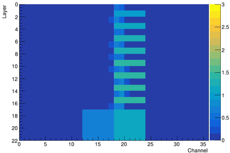
Beam profile for 140 GeV tagged MUON in a MUON beam
