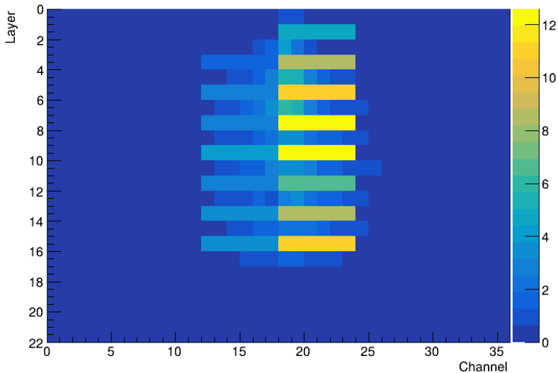
Beam profile for 25 GeV tagged ELECTRON in a MUON beam
