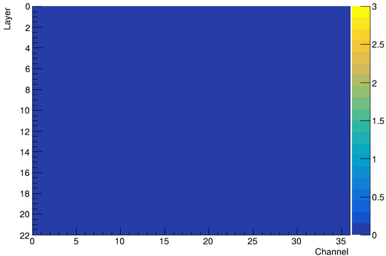
Beam profile for 160 GeV tagged MUON in a MUON beam
