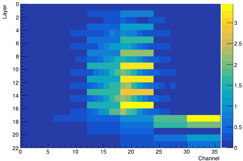
Beam profile for 160 GeV tagged EARLY_HADRON in a MUON beam
