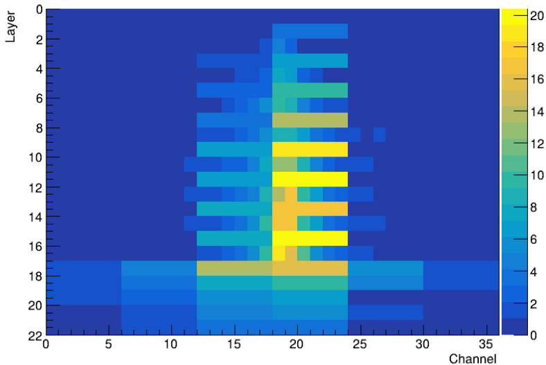
Beam profile for 140 GeV tagged EARLY_HADRON in a MUON beam
