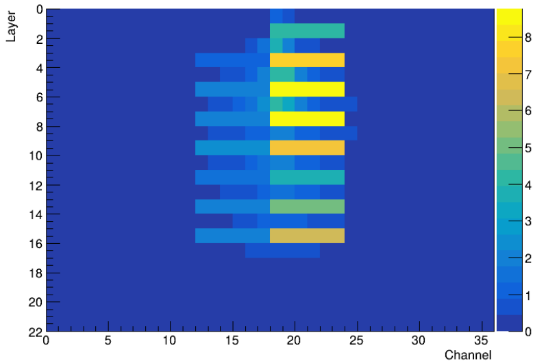
Beam profile for 15 GeV tagged ELECTRON in a MUON beam
