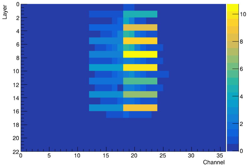
Beam profile for 20 GeV tagged ELECTRON in a MUON beam
