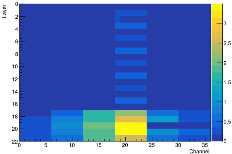
Beam profile for 240 GeV tagged LATE_HADRON in a MUON beam
