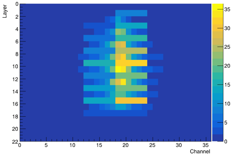
Beam profile for 180 GeV tagged ELECTRON in a MUON beam
