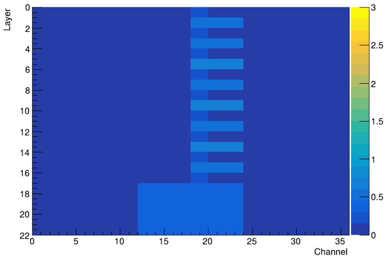
Beam profile for 25 GeV tagged MUON in a MUON beam
