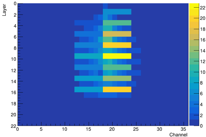
Beam profile for 50 GeV tagged ELECTRON in a MUON beam
