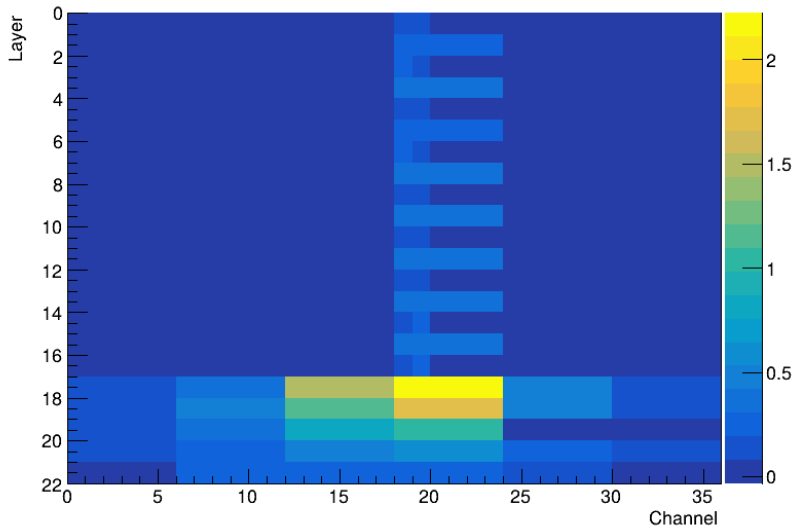
Beam profile for 20 GeV tagged LATE_HADRON in a MUON beam
