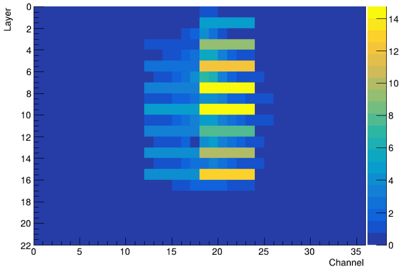
Beam profile for 30 GeV tagged ELECTRON in a MUON beam
