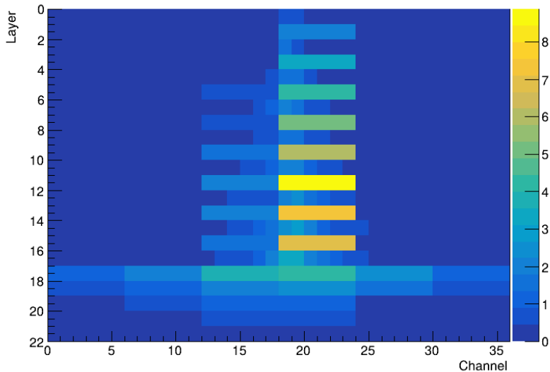
Beam profile for 25 GeV tagged EARLY_HADRON in a MUON beam
