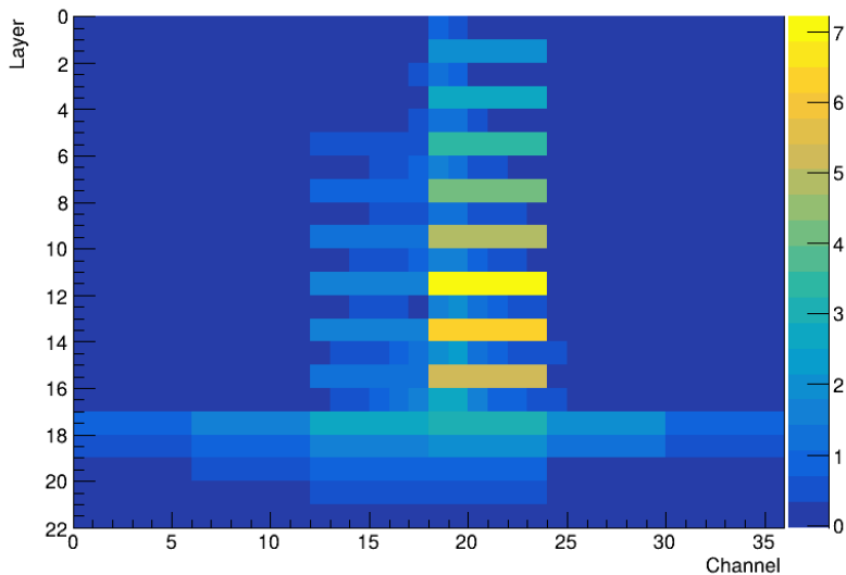
Beam profile for 20 GeV tagged EARLY_HADRON in a MUON beam
