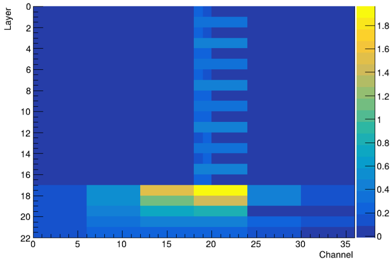
Beam profile for 15 GeV tagged LATE_HADRON in a MUON beam
