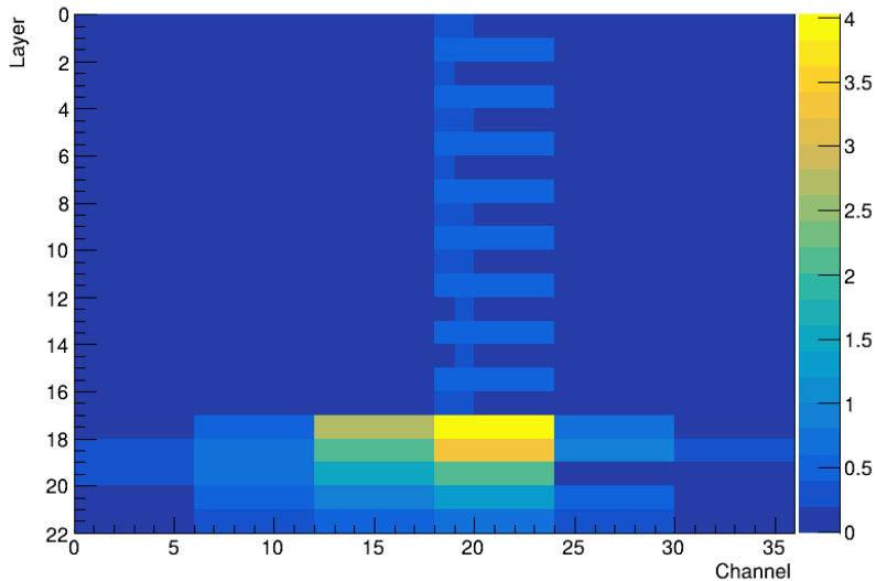
Beam profile for 25 GeV tagged LATE_HADRON in a MUON beam
