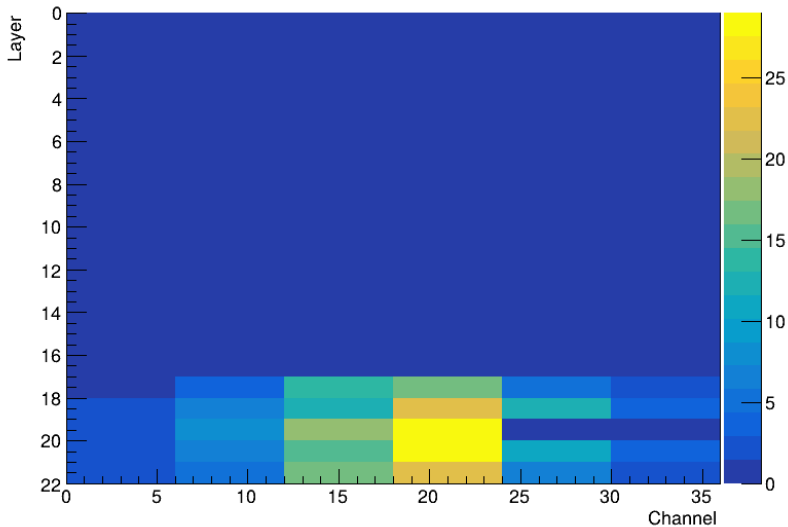
Beam profile for 300 GeV tagged LATE_HADRON in a MUON beam
