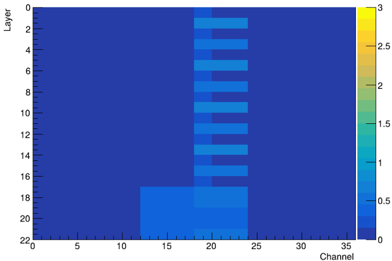
Beam profile for 30 GeV tagged MUON in a MUON beam
