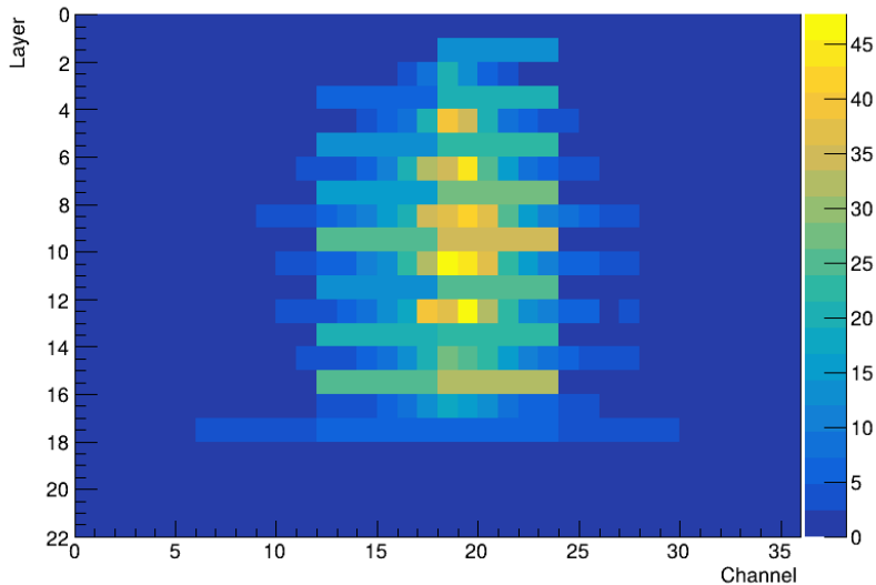
Beam profile for 240 GeV tagged ELECTRON in a MUON beam
