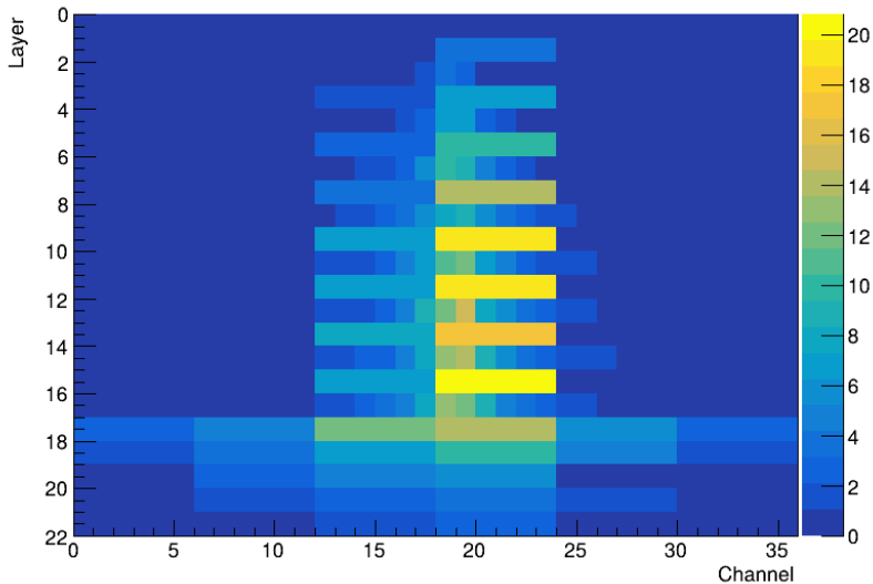
Beam profile for 100 GeV tagged EARLY_HADRON in a MUON beam
