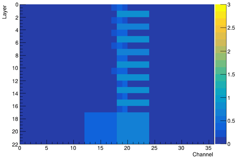
Beam profile for 50 GeV tagged MUON in a MUON beam
