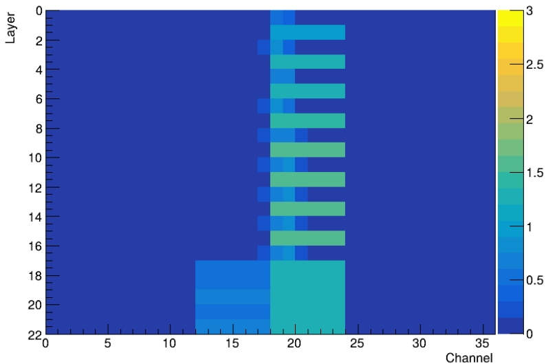
Beam profile for 240 GeV tagged MUON in a MUON beam
