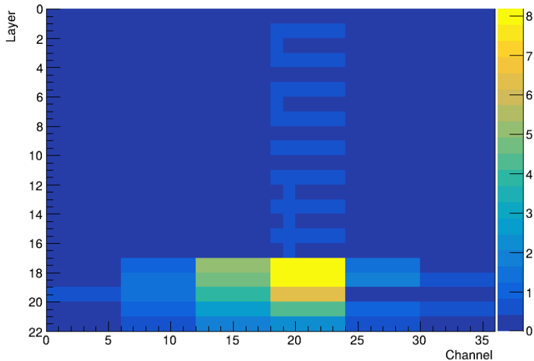
Beam profile for 50 GeV tagged LATE_HADRON in a MUON beam
