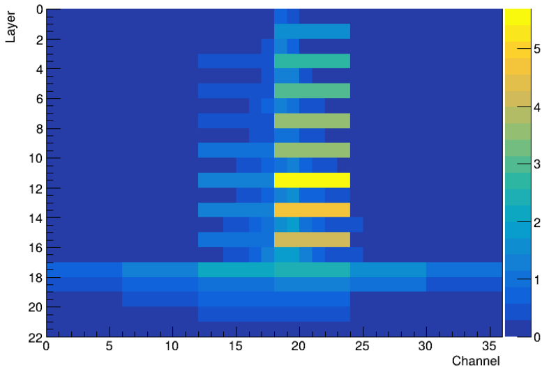
Beam profile for 15 GeV tagged EARLY_HADRON in a MUON beam
