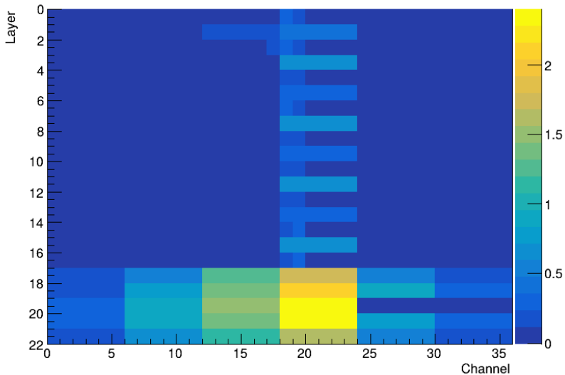
Beam profile for 180 GeV tagged LATE_HADRON in a MUON beam
