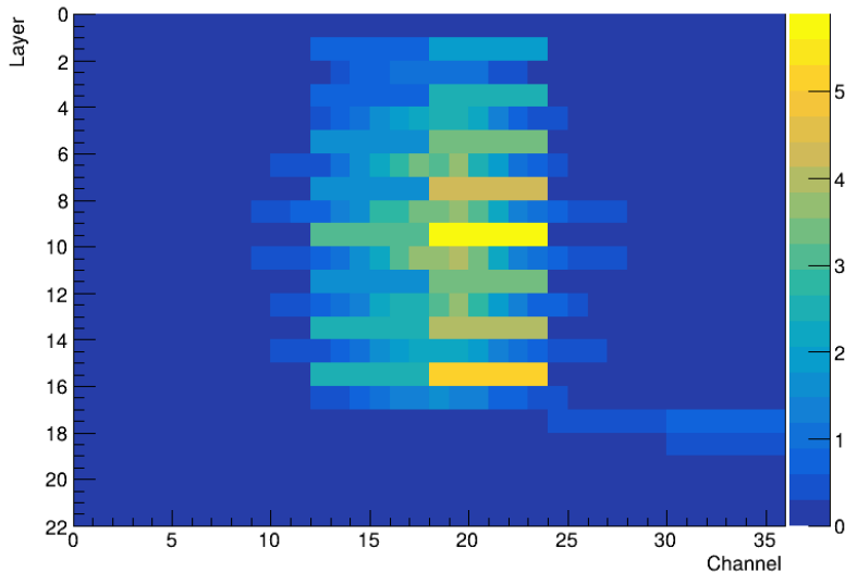
Beam profile for 160 GeV tagged ELECTRON in a MUON beam
