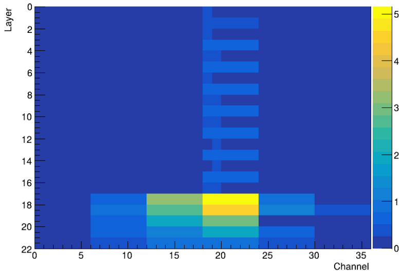
Beam profile for 30 GeV tagged LATE_HADRON in a MUON beam
