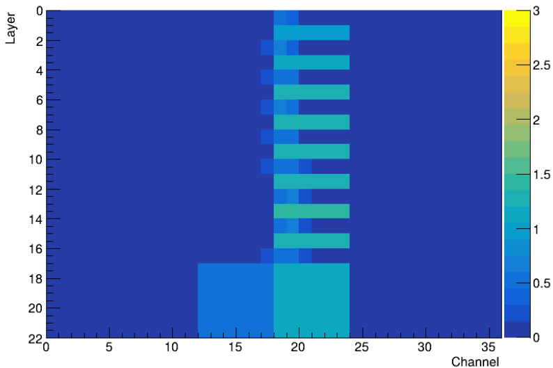
Beam profile for 100 GeV tagged MUON in a MUON beam
