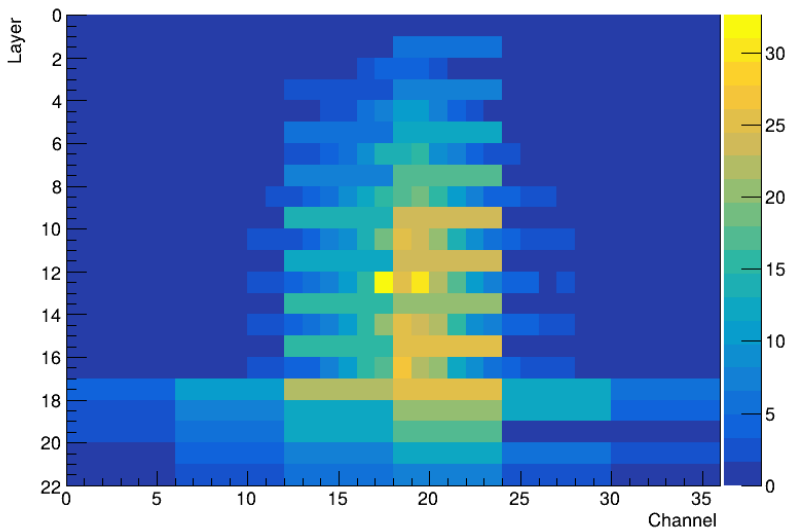
Beam profile for 300 GeV tagged EARLY_HADRON in a MUON beam
