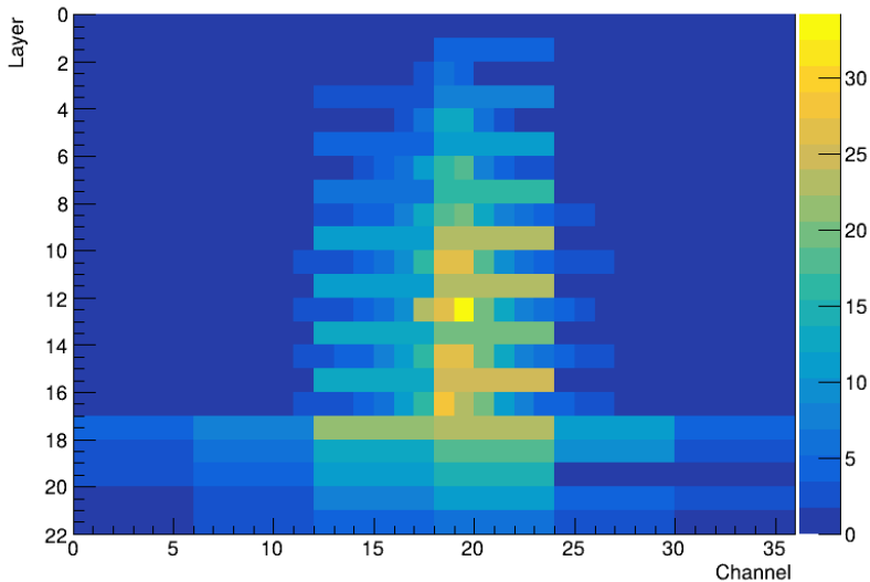
Beam profile for 240 GeV tagged EARLY_HADRON in a MUON beam
