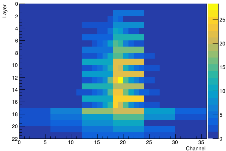
Beam profile for 180 GeV tagged EARLY_HADRON in a MUON beam
