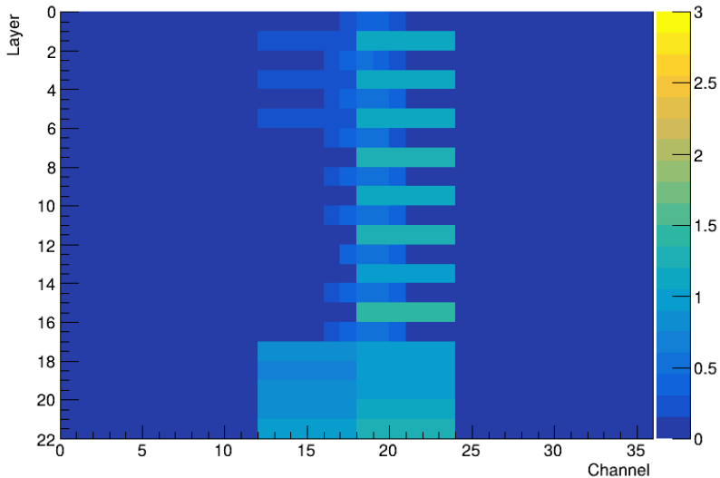
Beam profile for 300 GeV tagged MUON in a MUON beam
