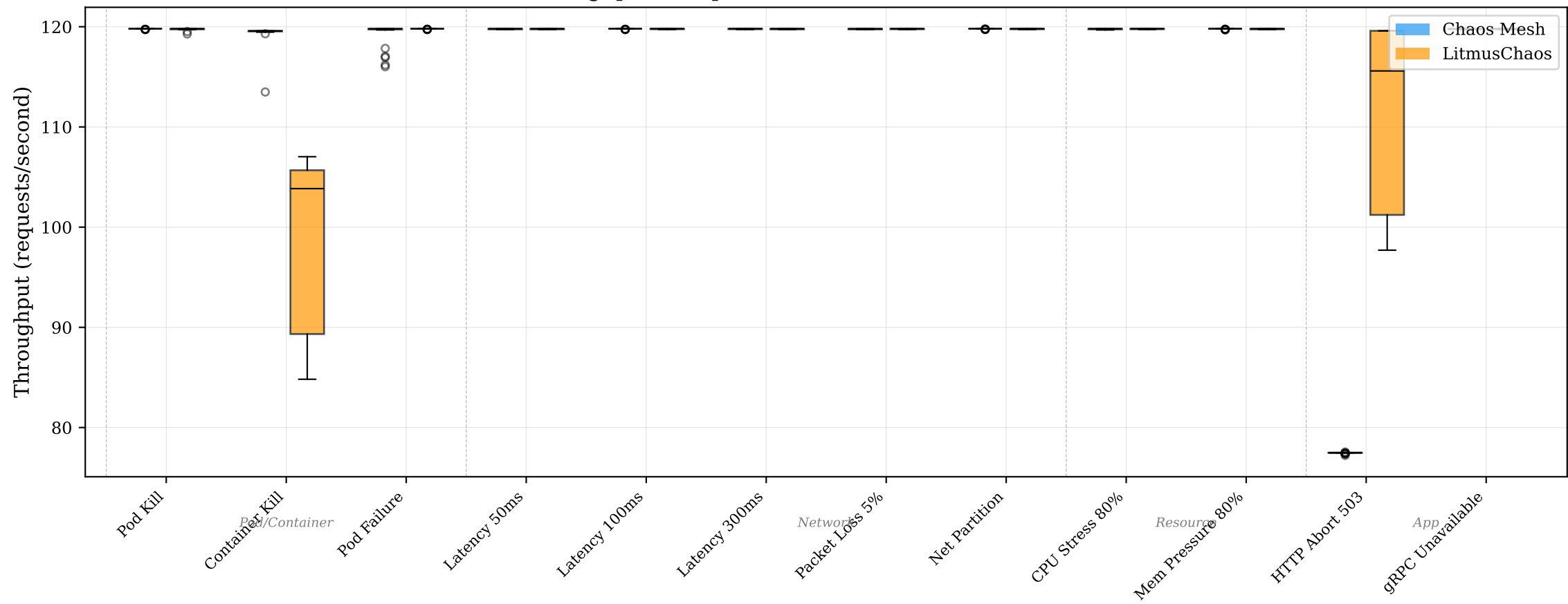
Throughput Comparison: Chaos Mesh vs LitmusChaos
