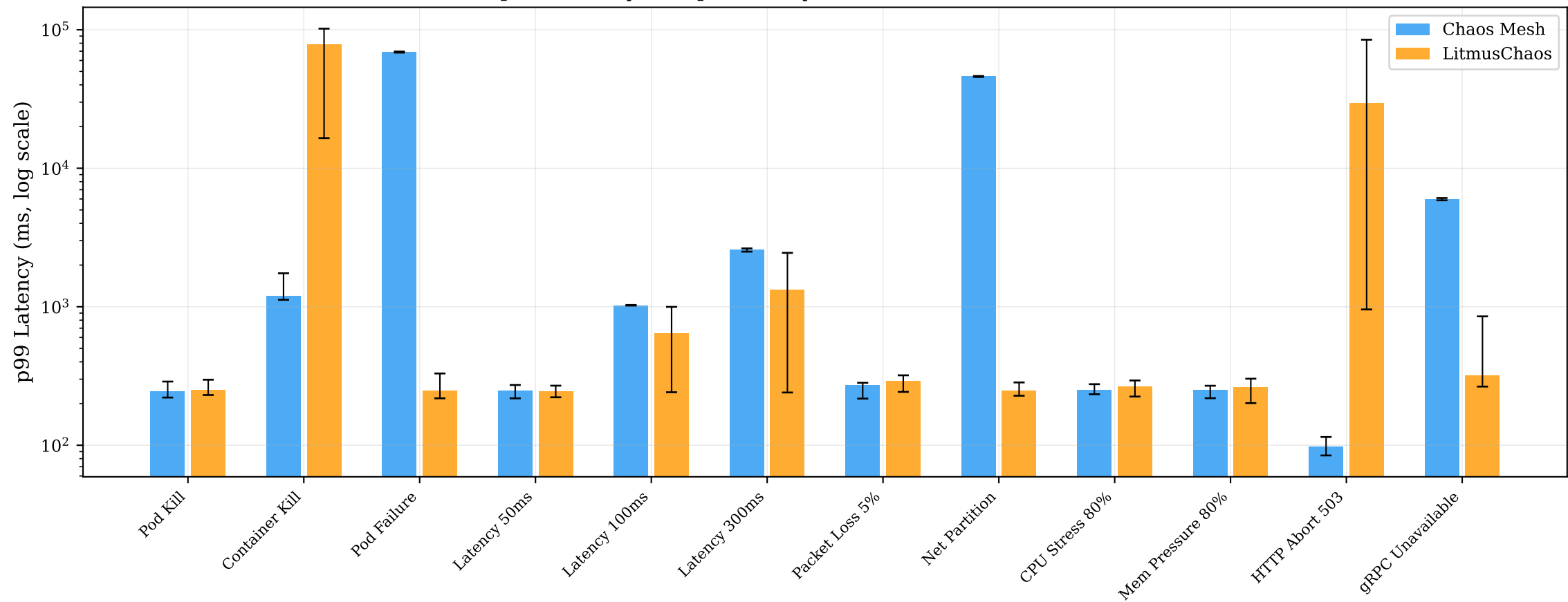
p99 Latency Comparison by Fault Scenario (median, IQR)
