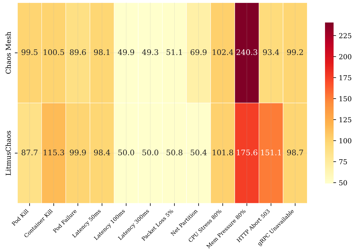
Memory Spike During Fault (MB)
