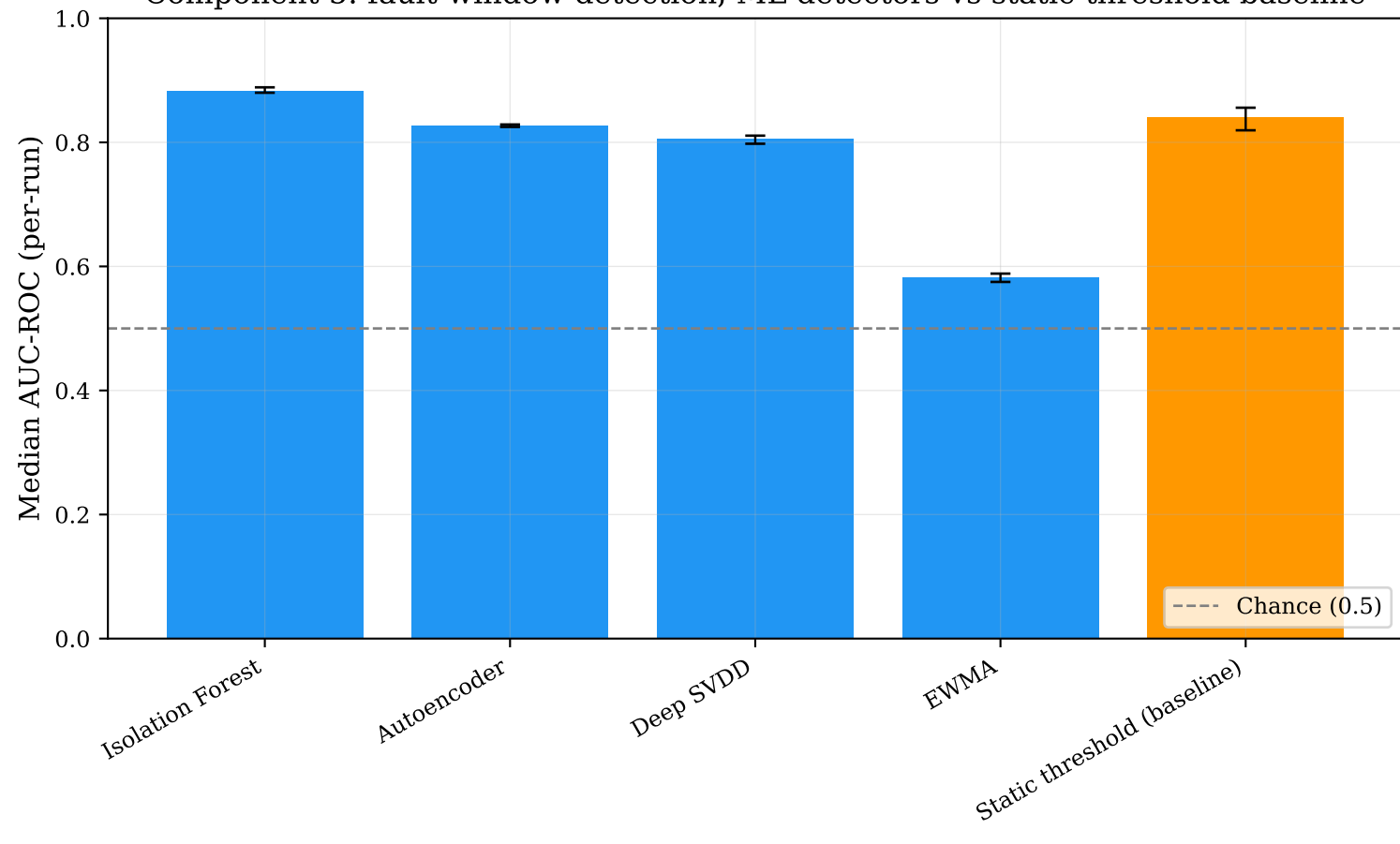
Component 5: fault-window detection, ML detectors vs static-threshold baseline
