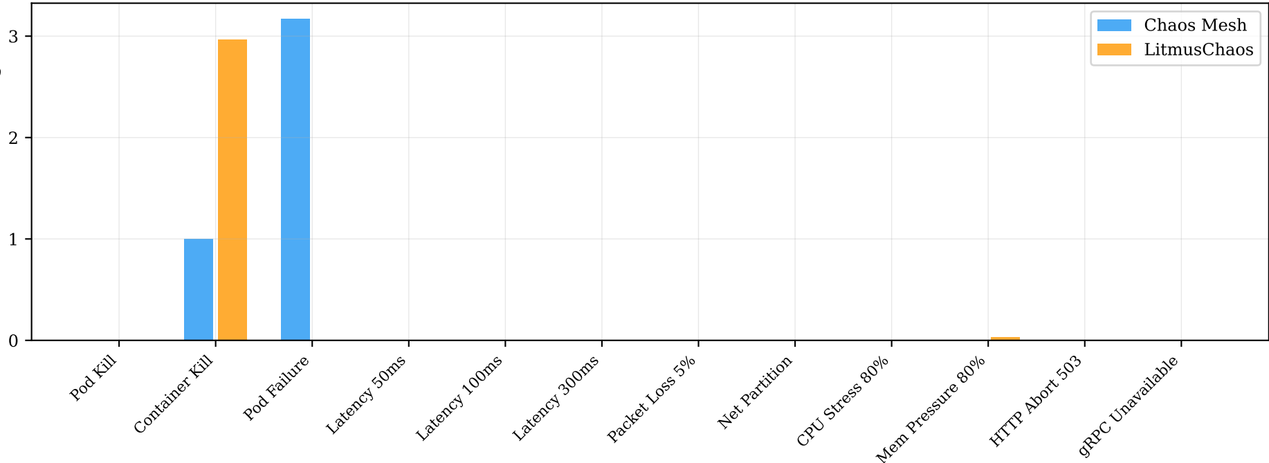
Pod Restarts by Fault Scenario
