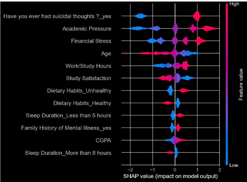
Figure 4.7 - SHAP Beeswarm: Full Model for Student Depression Dataset
