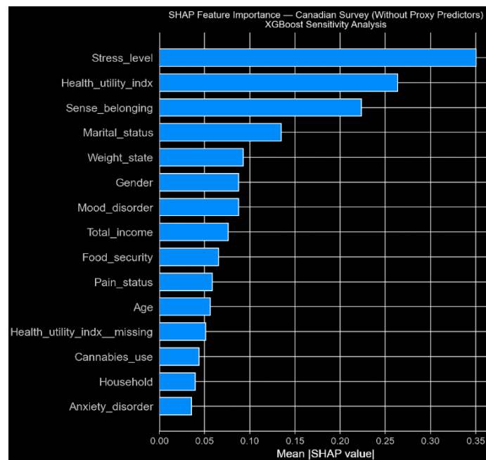
Figure 4.13 - SHAP Bar Plot: Sensitivity Analysis without Proxy Predictors for Canadian Survey Dataset
