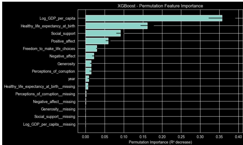
Figure 4.17 - XGBoost Permutation Feature Importance for Gallup World Happiness Report Dataset
