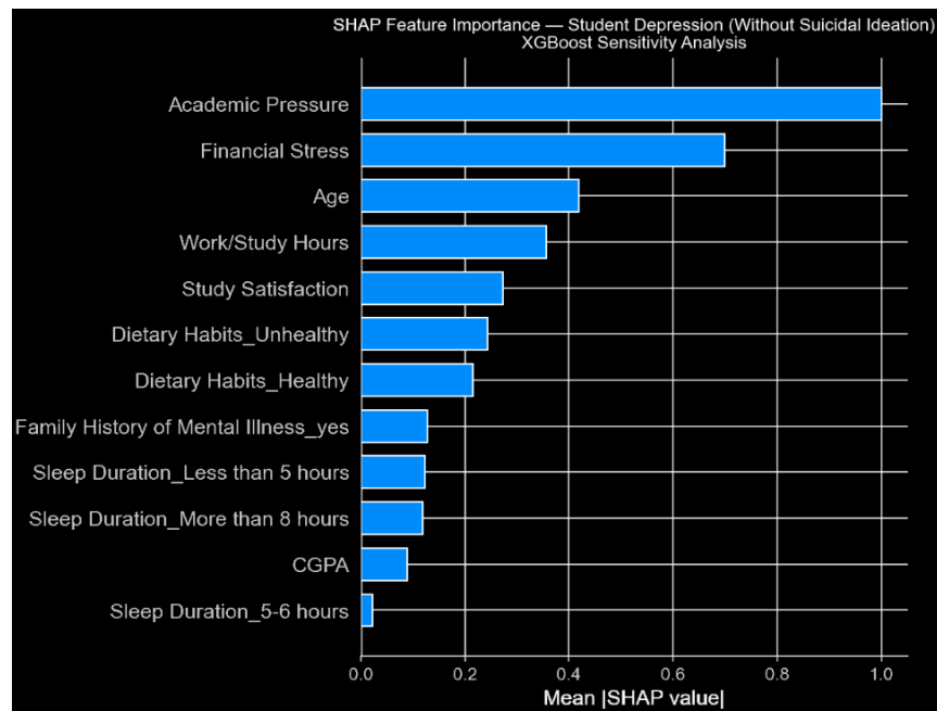
Figure 4.9 - SHAP Bar Plot: Sensitivity Analysis without Suicidal Ideation for Student Depression Dataset
