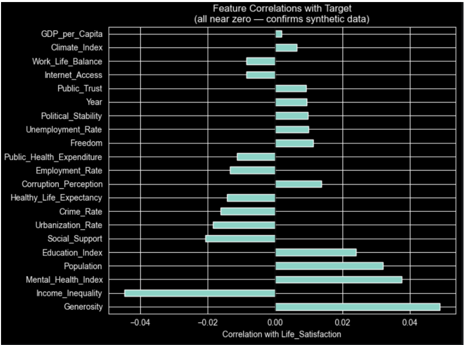
Figure 4.15 - Feature Correlation Chart for Synthetic World Happiness Report Dataset
