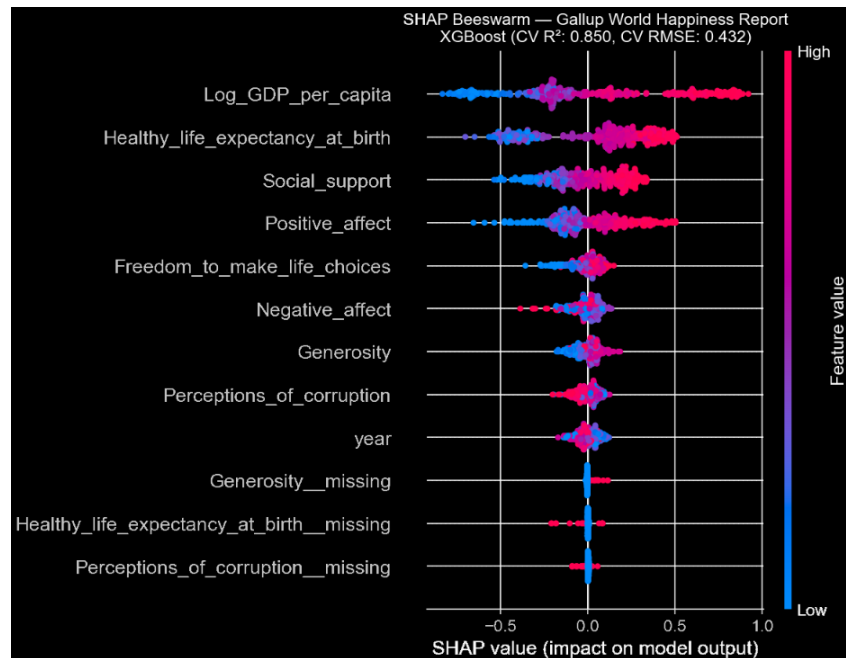
Figure 4.19 - SHAP Beeswarm: Full Model for Gallup World Happiness Report Dataset
