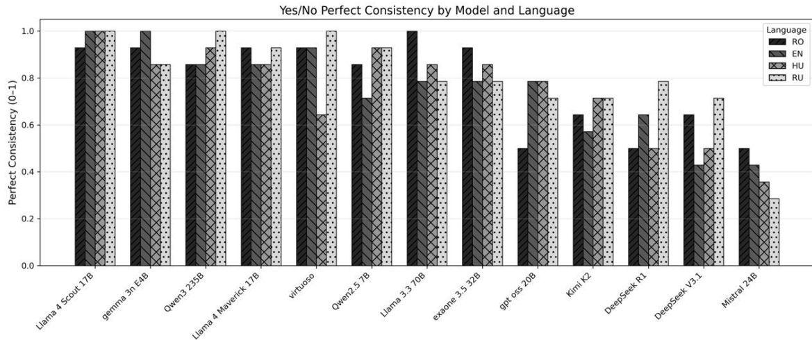
Figure 5: This figure shows the perfect consistency of "Yes" and "No" responses within each model across multiple runs and languages (languages from left to right: Romanian, English, Hungarian and Russian). A perfectly consistent model would always give the same "Yes" or "No" answer for a given question in a given language across all runs.
