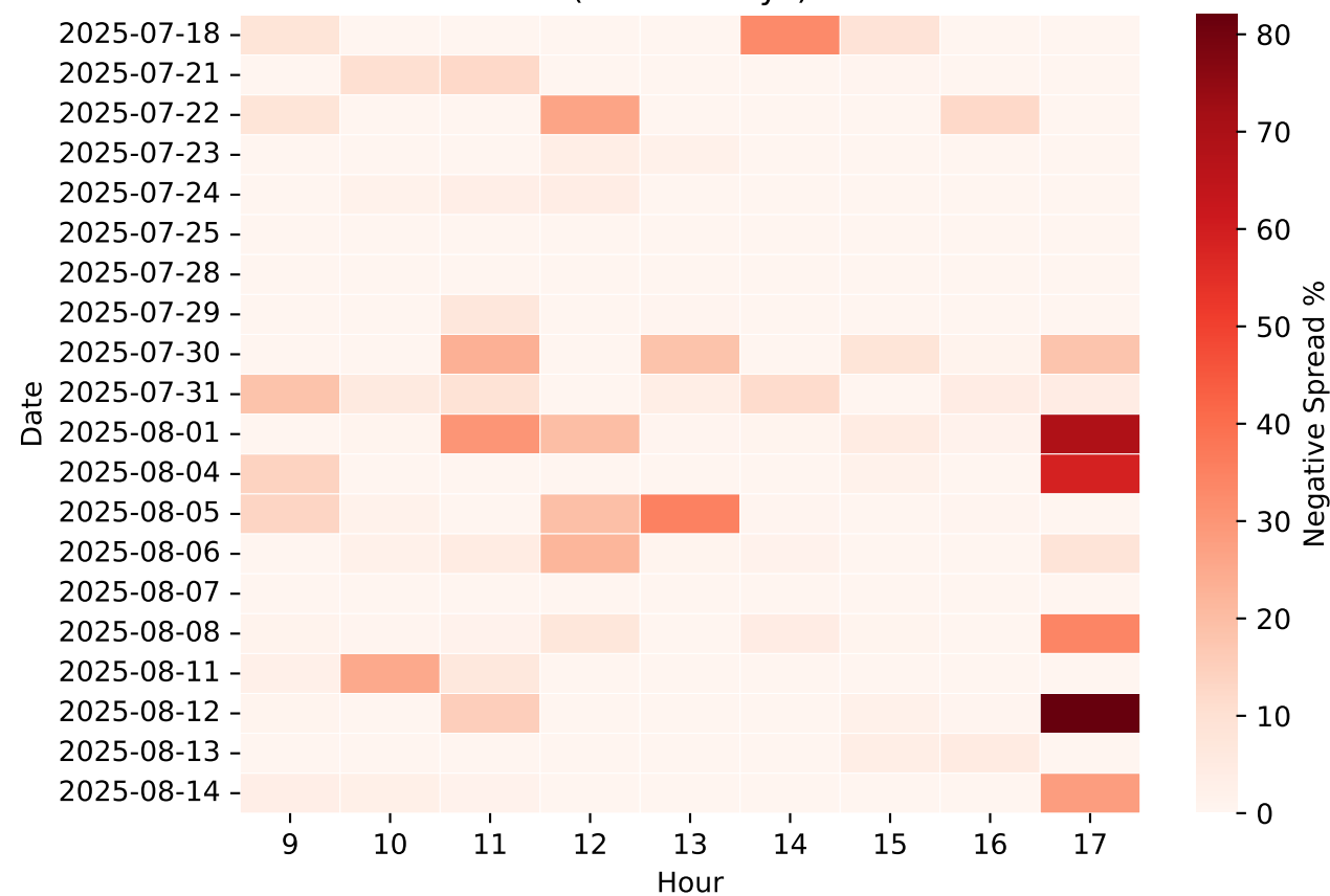
Negative Spread % Heatmap (Last 20 days)
