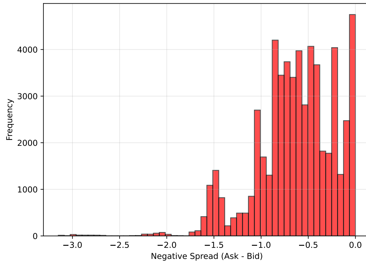
Distribution of Negative Spreads (57,969 records)
