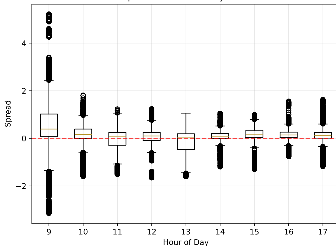
Spread Distribution by Hour
