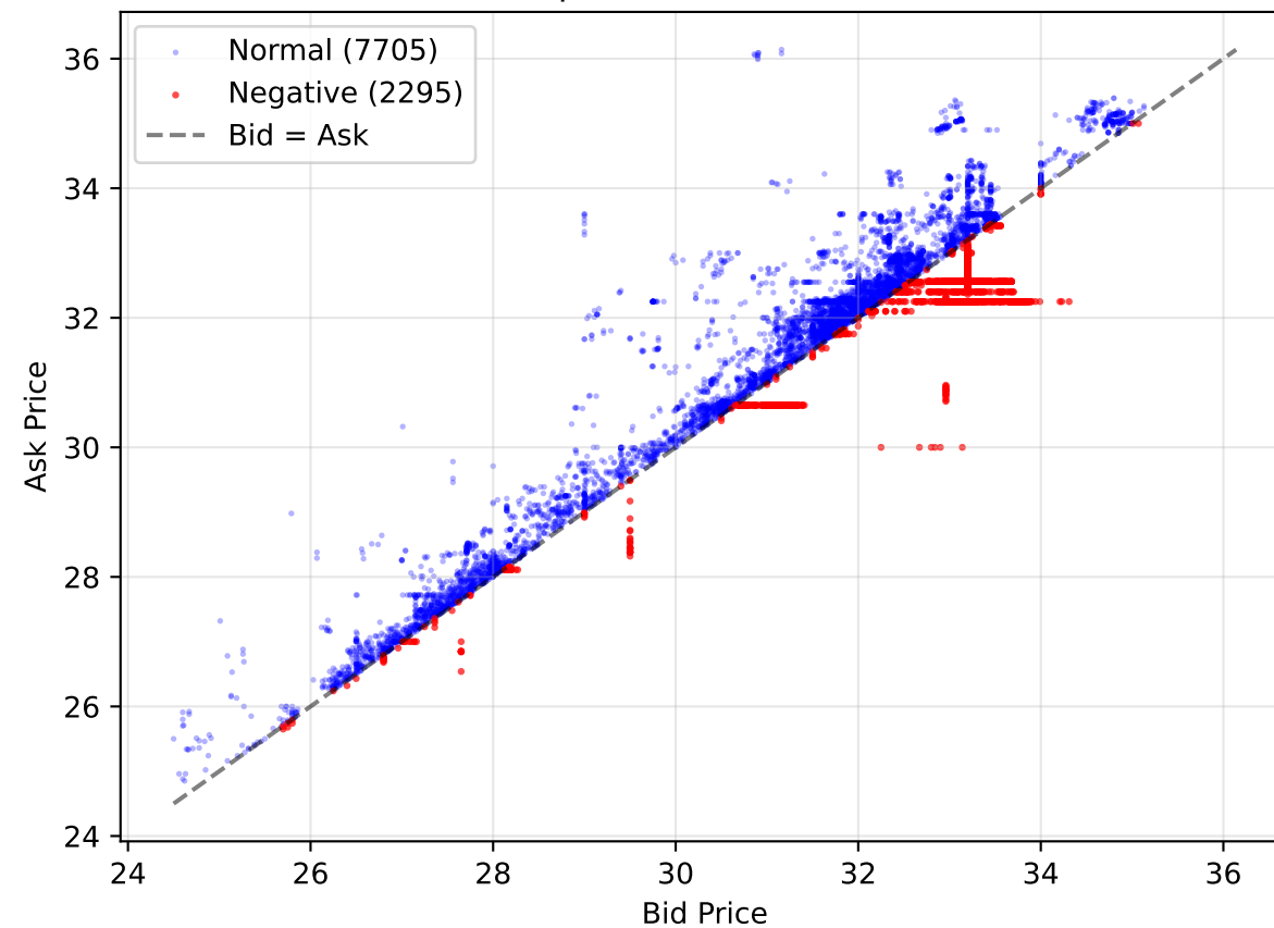
Bid vs Ask Prices (Sample of 10,000 records)
