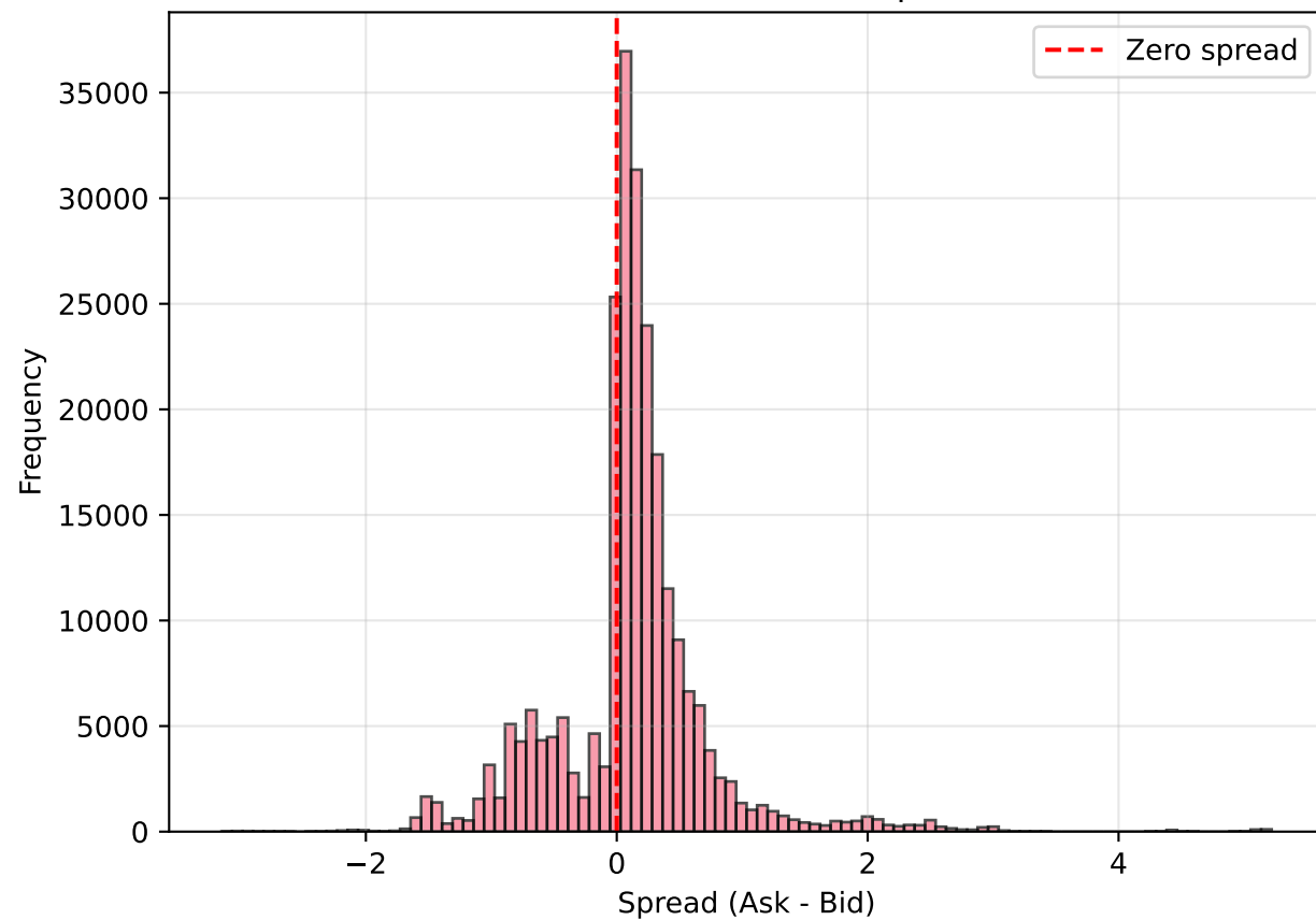
Distribution of Bid-Ask Spreads
