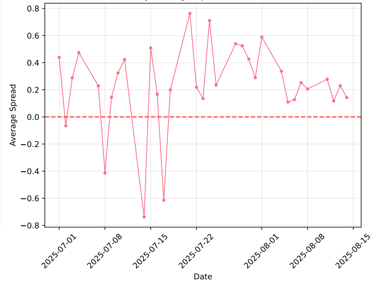
Daily Average Spread Over Time
