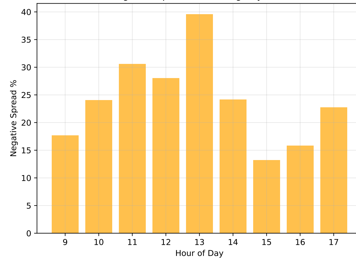
Negative Spread Percentage by Hour
