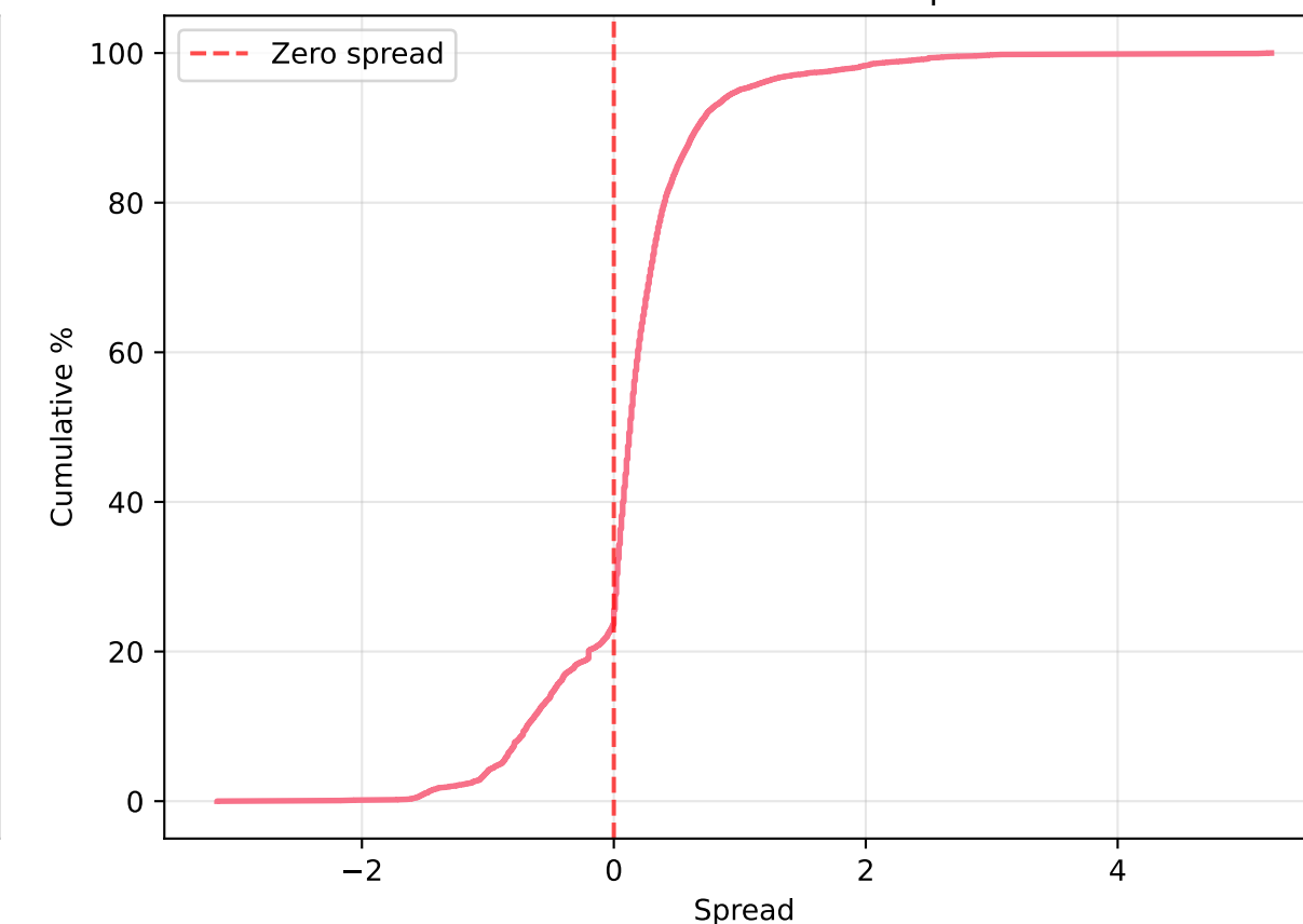
Cumulative Distribution of Spreads
