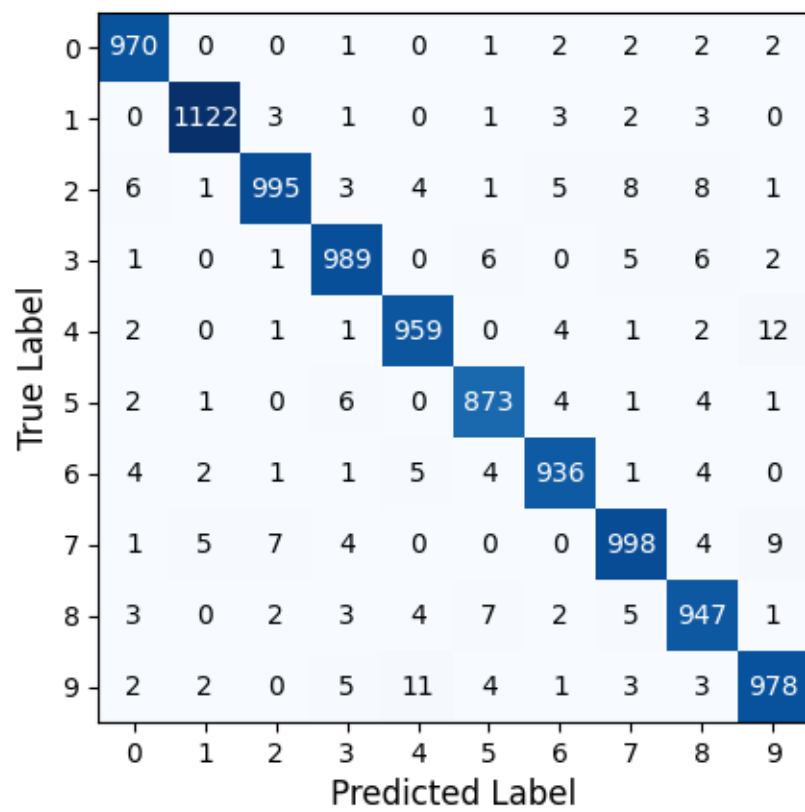
Figure 1: Confusion matrix for Question 3.6
