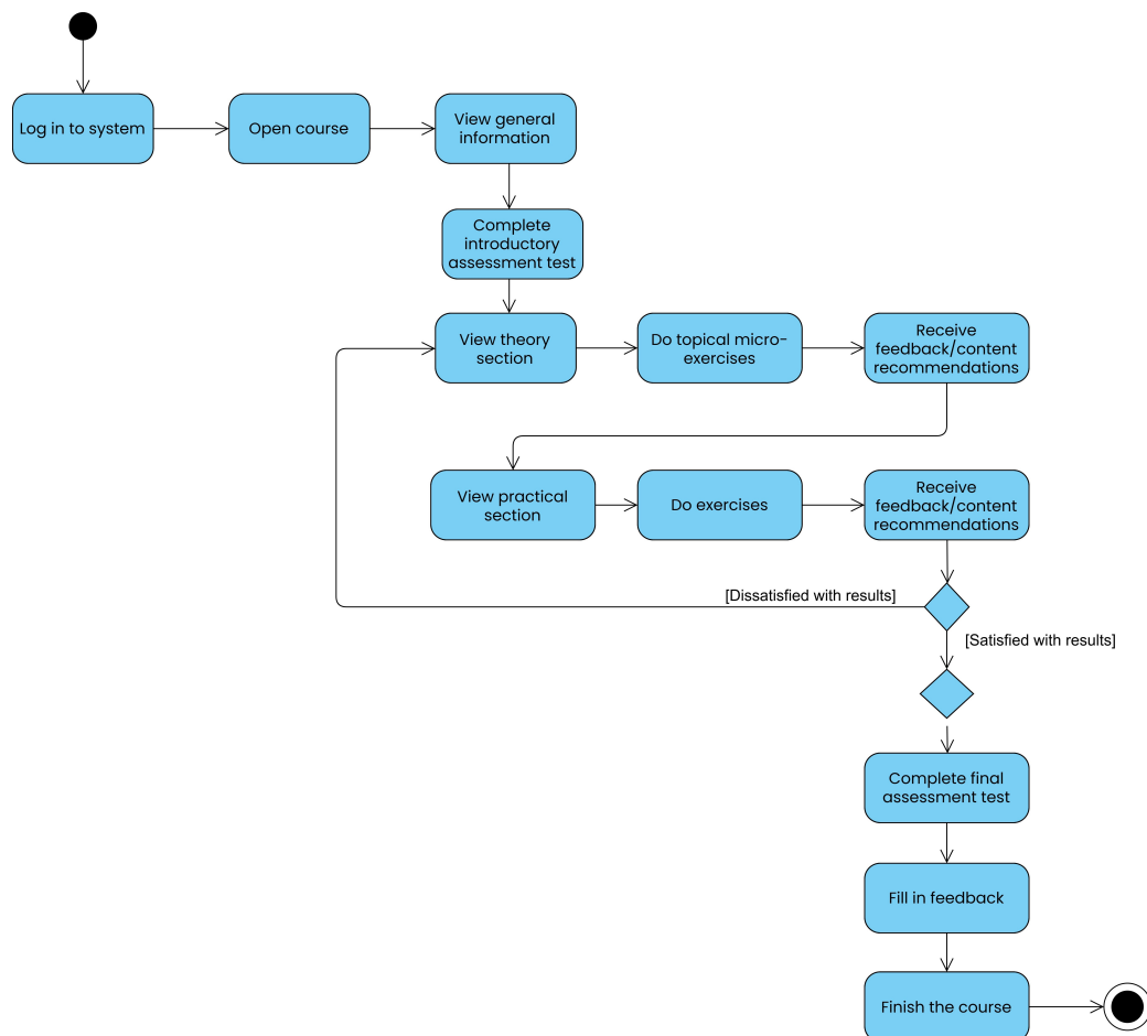
Figure 6.2: Activity diagram from a student's perspective.
