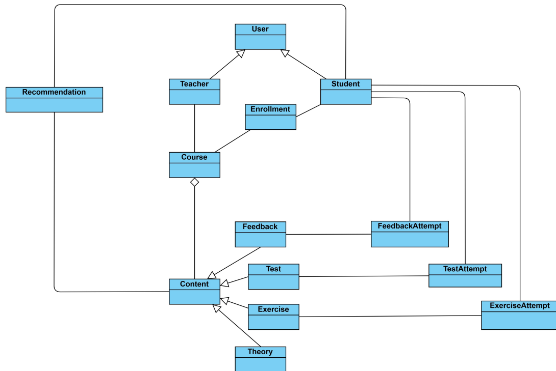
Figure 6.1: Class diagram of the designed system.
