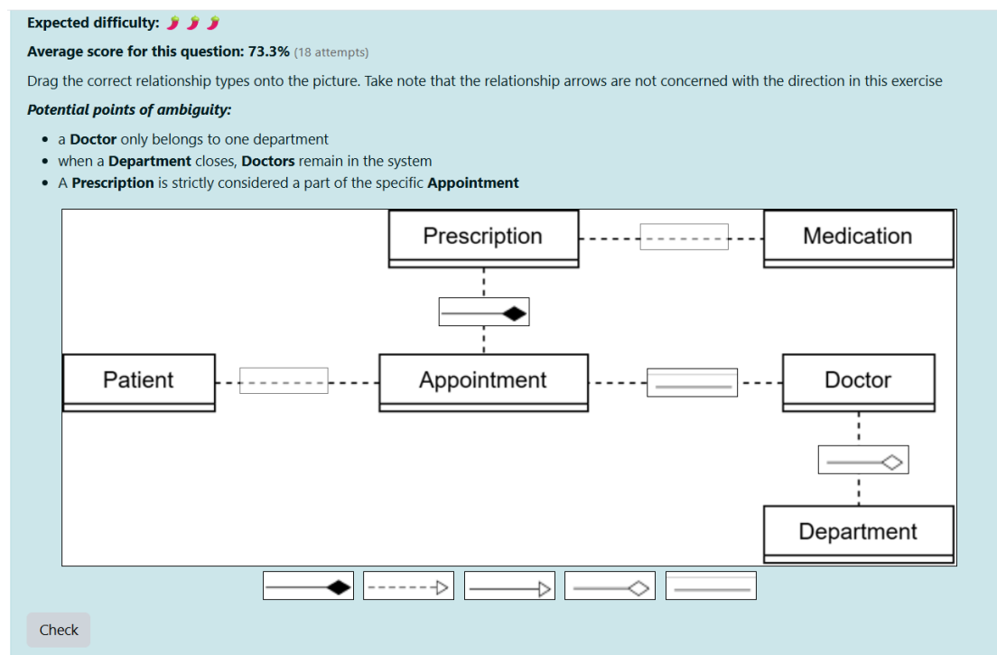
Figure 7.5: Simulating modeling with the drag and drop onto picture activity
