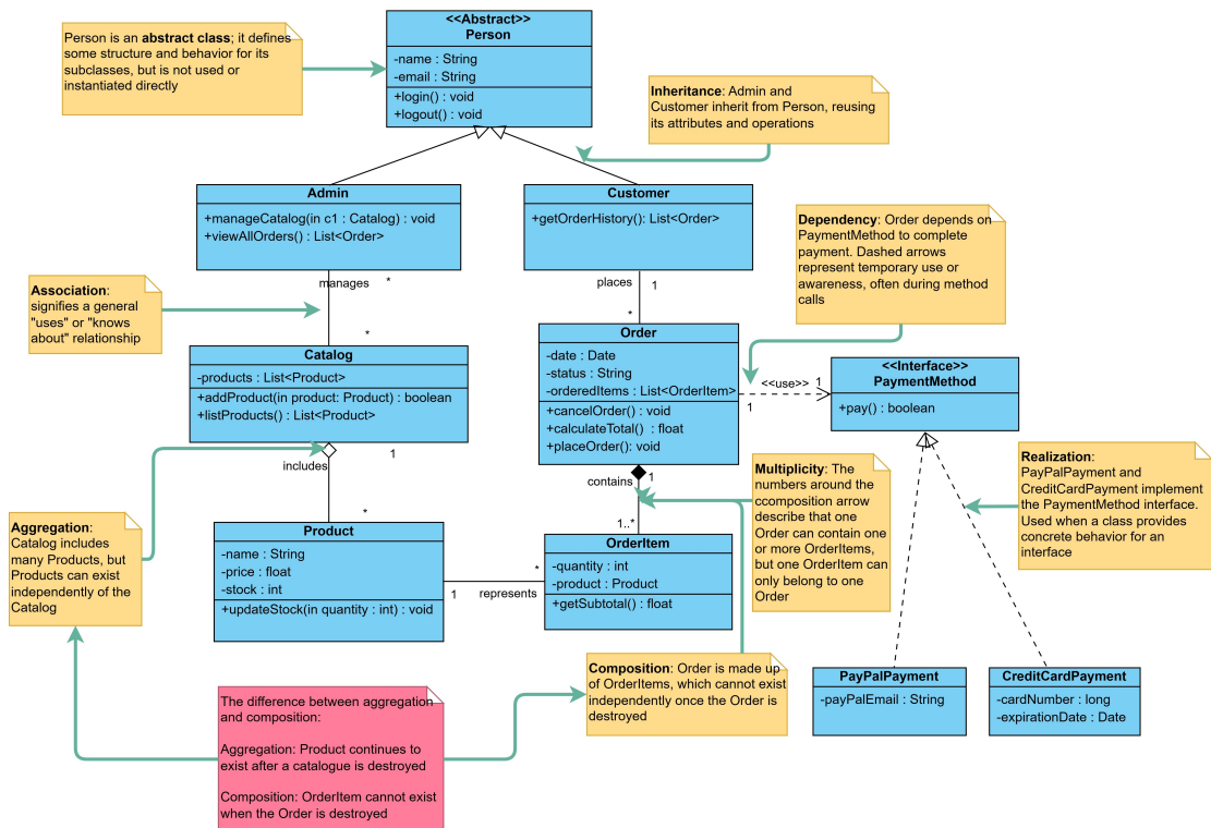
Figure 2.3: An example of a class diagram.
