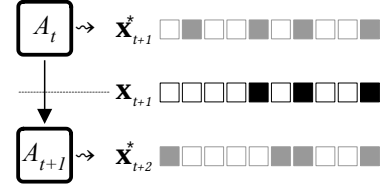
Fig. 2. Iterative adaptation in discrete time. Following input \mathbf{x}_t , the system A_t issues the prediction \mathbf{x}_{t+1}^* . Upon observing the realised input \mathbf{x}_{t+1} , it updates in response to the error in the second bit and produces the next one-step-ahead prediction \mathbf{x}_{t+2}^* .
