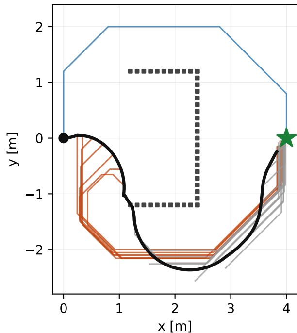
(a) as deployed — A* re-plans with no memory
