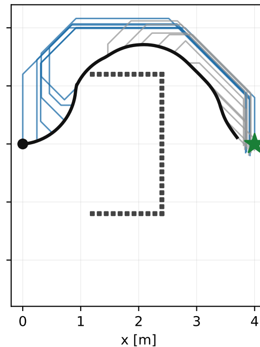
(b) with pre-selection, \delta = 0.5 m
