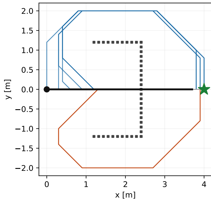
(a) as deployed — A* re-plans with no memory
