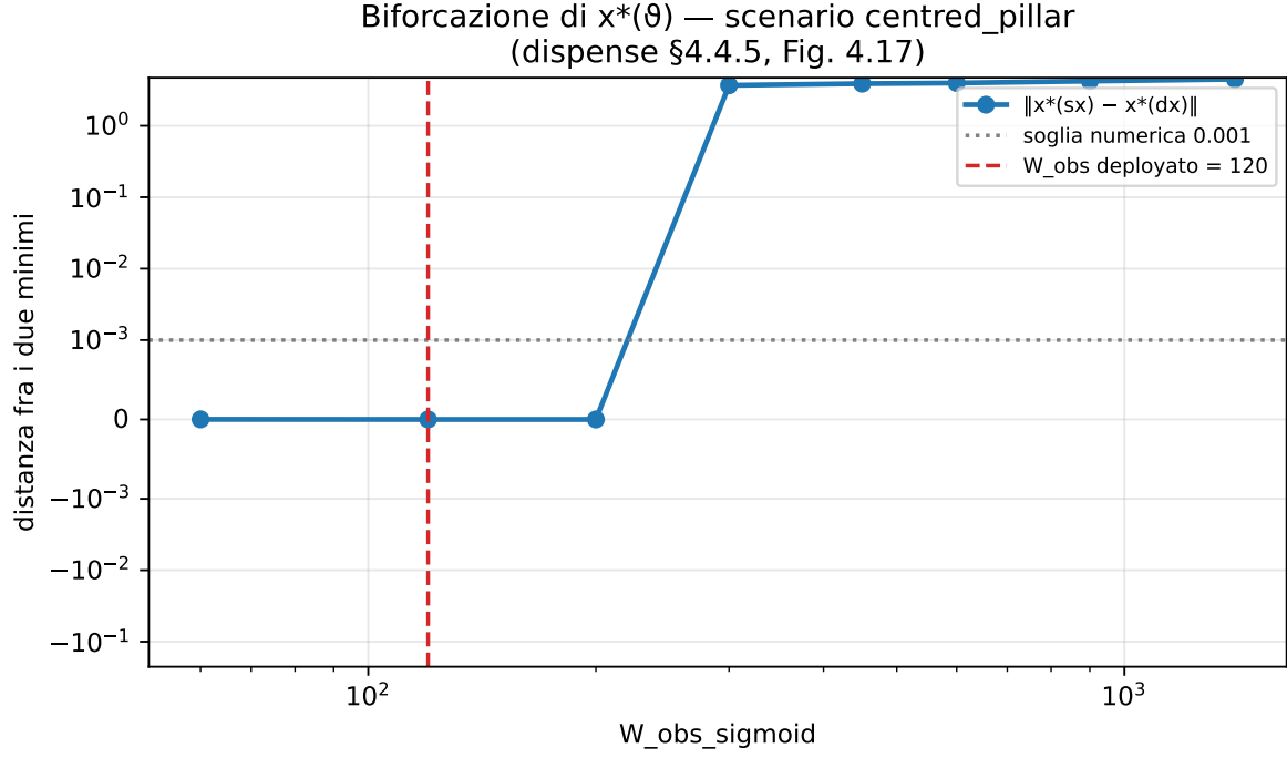
Figure 2: Separation between the trajectories returned from a left-biased and a right-biased initial guess, against the obstacle weight W_{\text{obs}} . Below the transition the two guesses collapse onto the same minimum and the control law is a regular function of the state; above it they do not.
