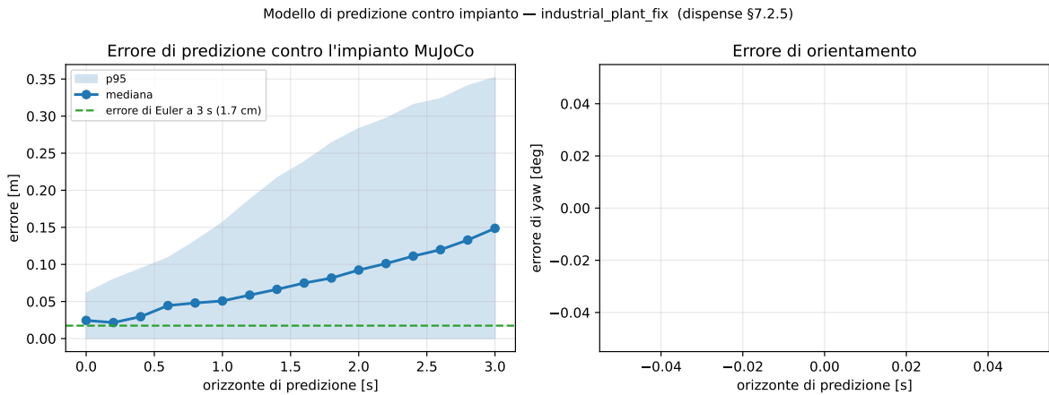
Figure 1: Prediction error against the position along the horizon, over 775 cycles of the recorded run industrial_plant_fix : median and 95th percentile. The residual at k = 0 is time misalignment between the instant the prediction is published and the instant the pose is sampled, not model error, and is subtracted before quoting the divergence.
