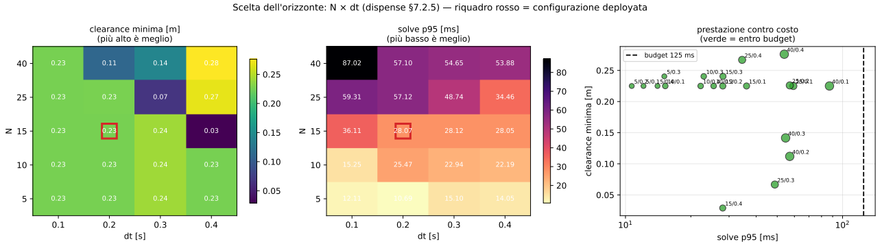
Figure 3: Joint sweep of the prediction horizon N and the sampling time \Delta t in closed loop. The deployed configuration is marked. Cost is governed by N ; closed-loop quality is governed by the product N\Delta t , and not monotonically.
