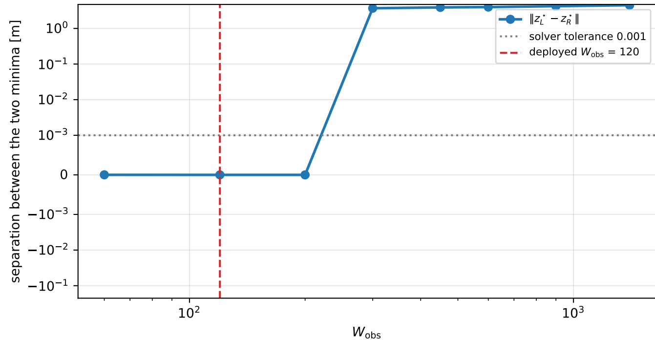
Bifurcation of z^*(\theta) --- scenario centred_pillar (dispense §4.4.5, Fig. 4.17)
