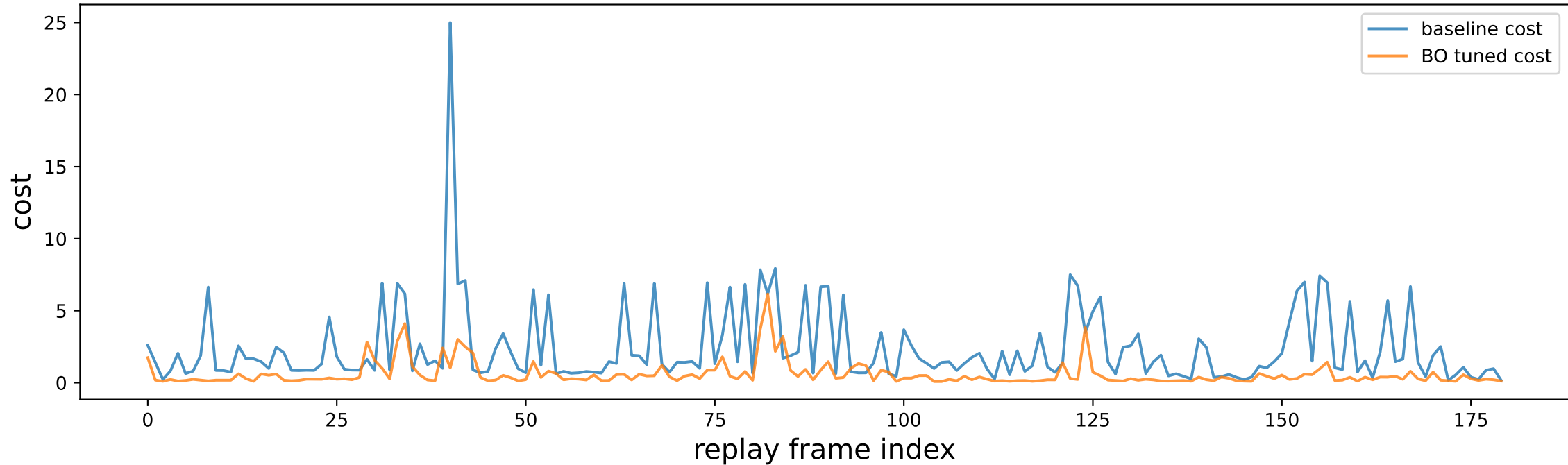
Per-frame MPC step cost after optimization
