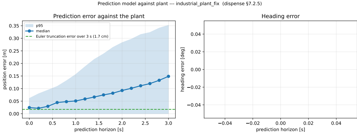
Figure 2: Prediction error against the position along the horizon, over 775 cycles of the recorded run industrial_plant_fix : median and 95th percentile. The residual at k = 0 is time misalignment between the instant the prediction is published and the instant the pose is sampled, not model error, and is subtracted before quoting the divergence.
