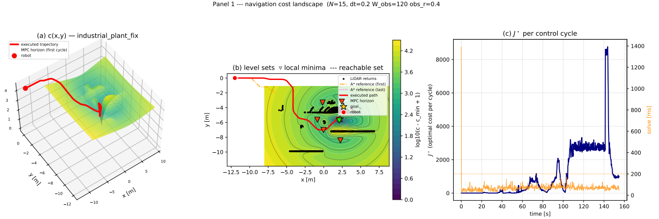
Figure 1: The navigation cost landscape of the recorded run industrial_plant_fix . (a) the surface c(p) of Eq. (26) over the world plane, with the executed trajectory (red) and one MPC horizon (dashed) drawn on the surface: the obstacle term raises a ridge along every wall of the plant, the tracking term forms the valley along the A^* reference. (b) the same field as level sets, with the local minima marked and the shaded region showing the set reachable within one horizon under \mathcal{U} — the constraint, not the cost, is what excludes most of the plane. (c) the optimal cost J^* of each control cycle, and the solve time beside it. The point worth noticing is in panel (a): the trajectory does not follow steepest descent , and climbs the surface wherever doing so lowers the sum over the horizon.
