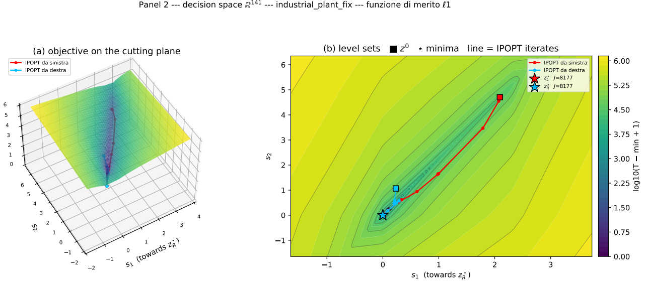
Figure 4: The objective in the decision space \mathbb{R}^{141} , on a plane constructed to contain both local minima of the recorded cycle. (a) the surface; (b) its level sets with the two minima ( \star ), the initial iterate ( \blacksquare ) and the IPOPT iterates joining them. What is plotted is not the objective f but the \ell^1 merit function T_1(z) = f(z) + \sigma \|c(z)\|_1 : in the simultaneous parametrisation X and U are independent variables tied by the dynamic equalities, so a generic point of the plane is not dynamically feasible and a plot of f alone would show a landscape the solver never traverses. The merit function is what the line search actually decreases.
