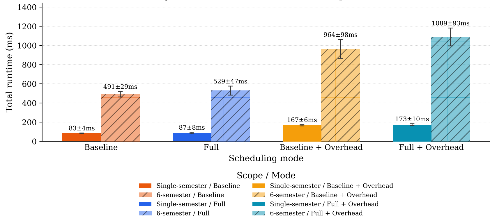
Single-semester vs 6-semester: runtime per mode
