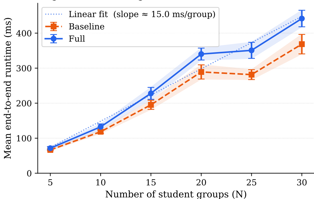
Fig. 4 — Scheduling runtime vs. N (includes DB I/O)
