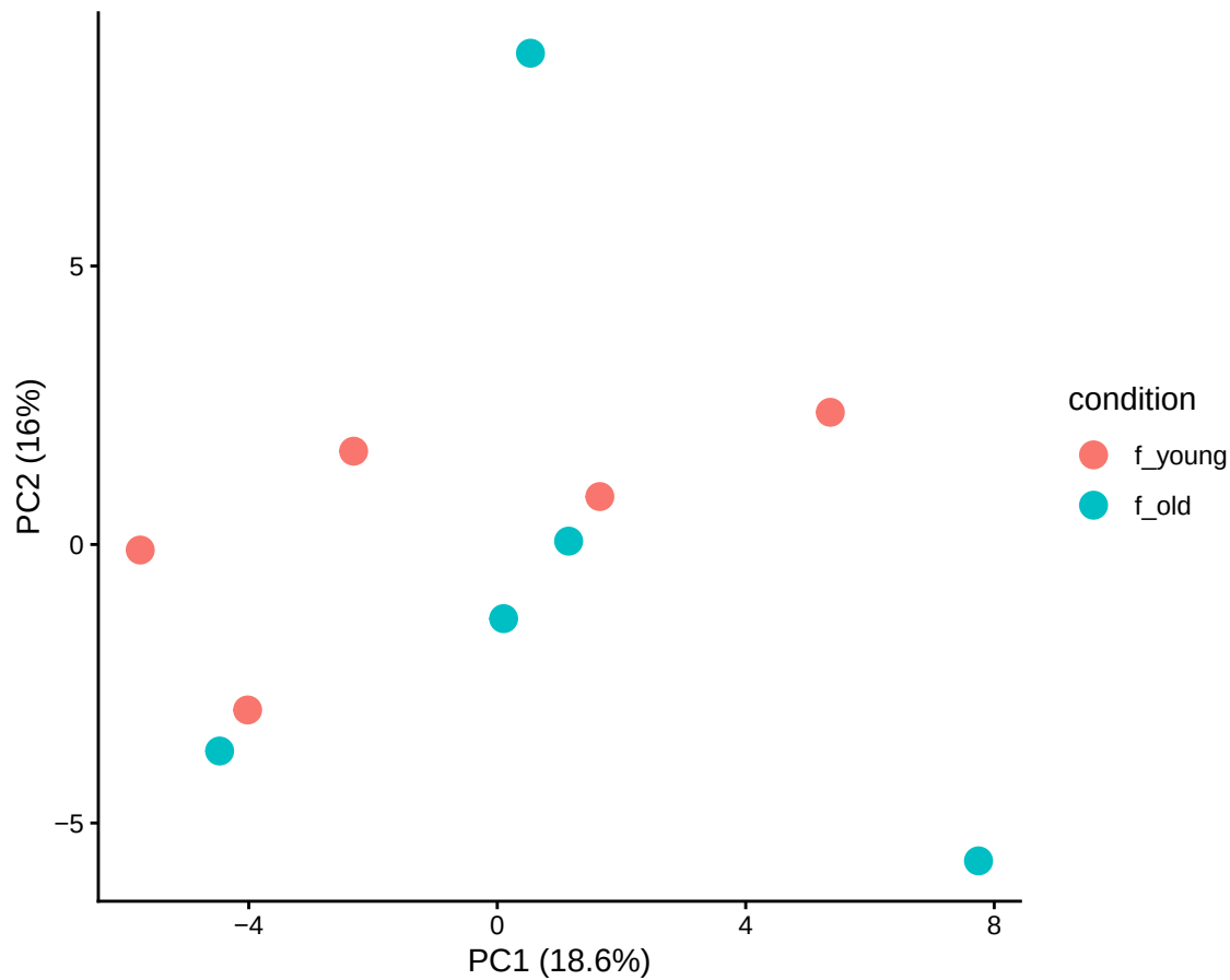
hisat2_PE edgeR, top 100 genes
