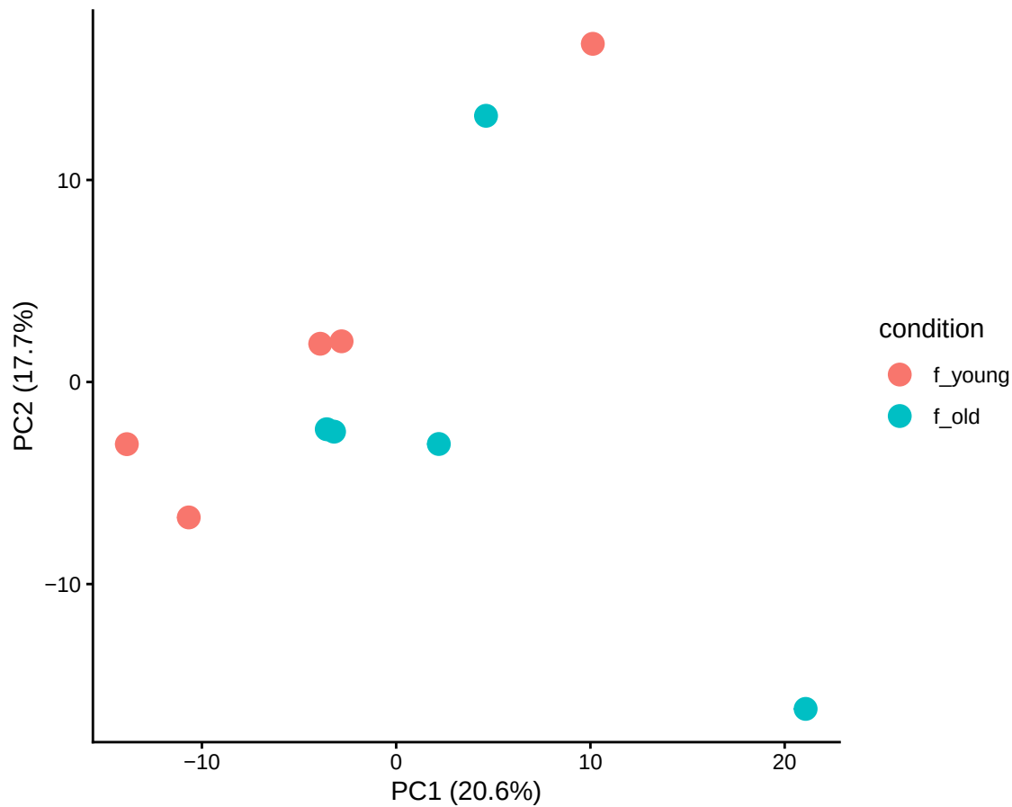
star_PE edgeR, top 500 genes
