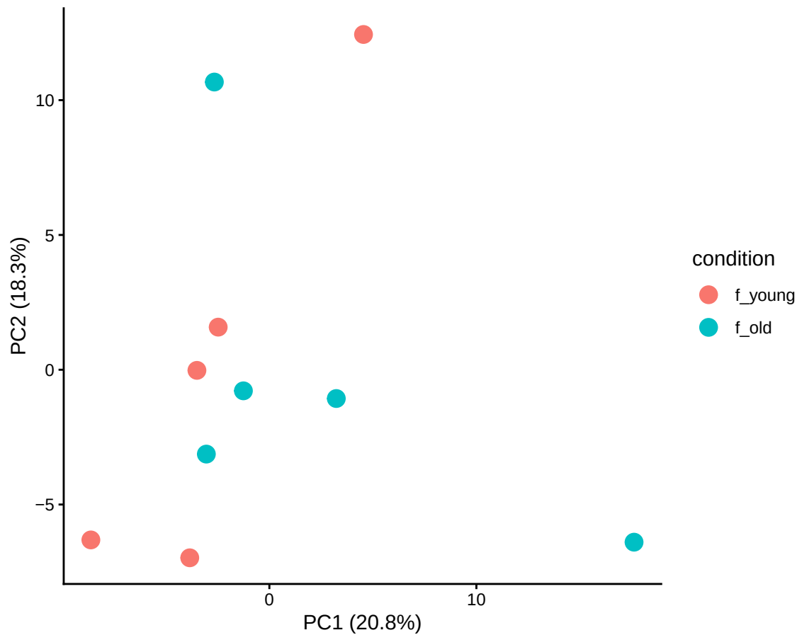
hisat2_PE edgeR, top 250 genes
