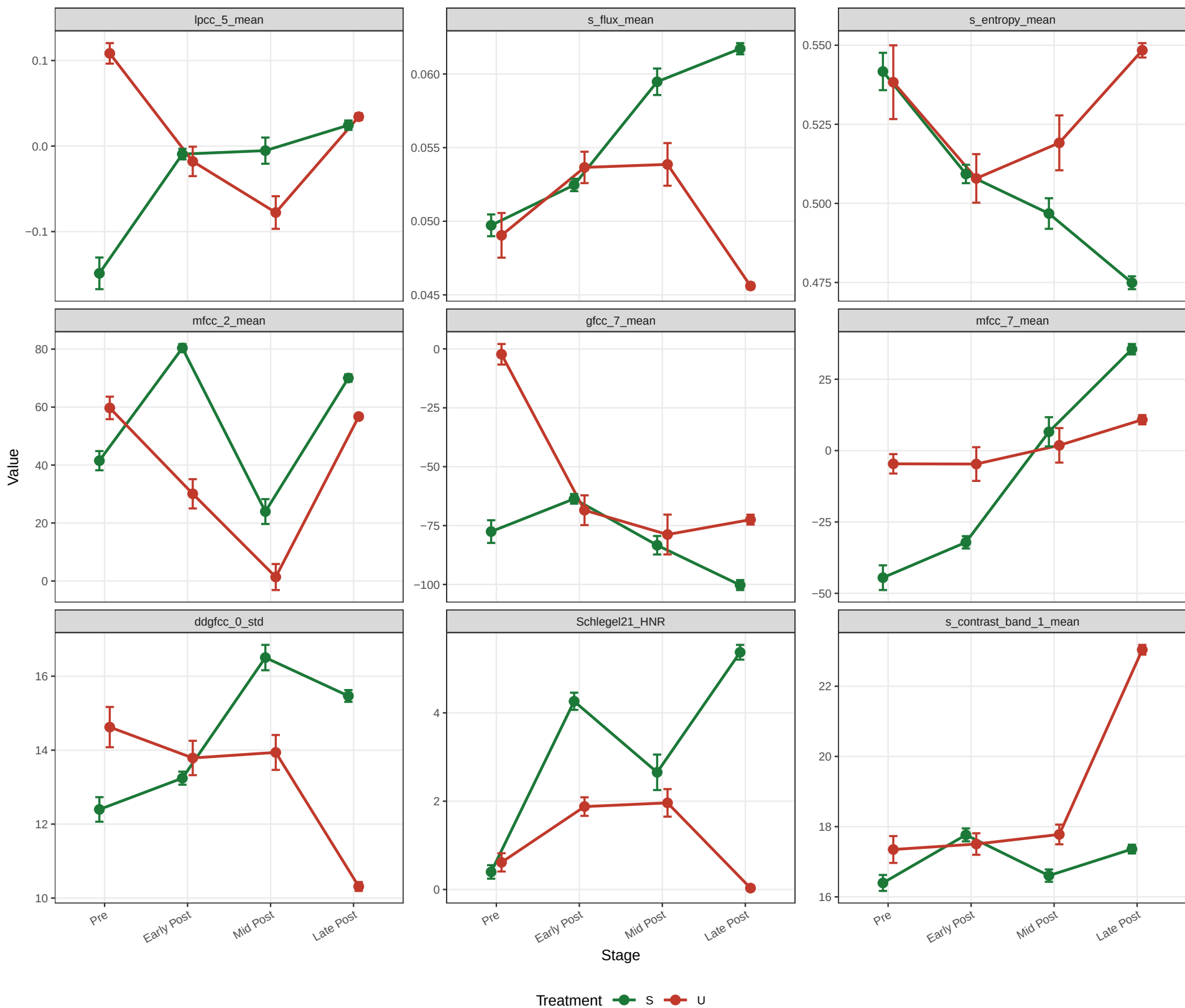
Top 9 features by Stage \times Treatment interaction p-value
