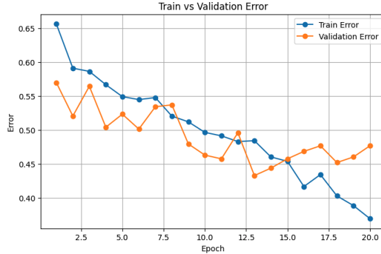
Figure 5: Training and Validation Error of the Primary Model
