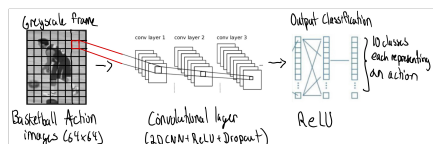
Figure 3: Architecture of the Baseline Model
