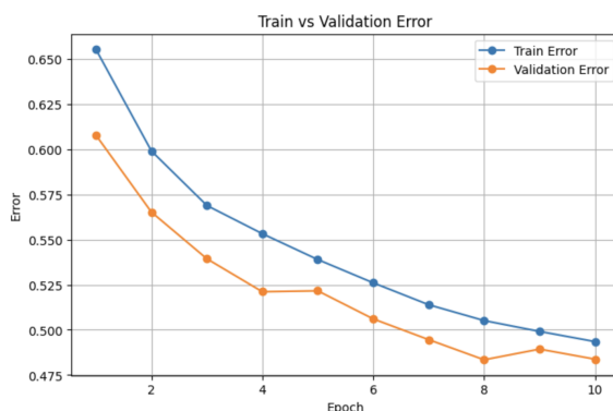
Figure 4: Training and Validation Error of the Baseline Model
