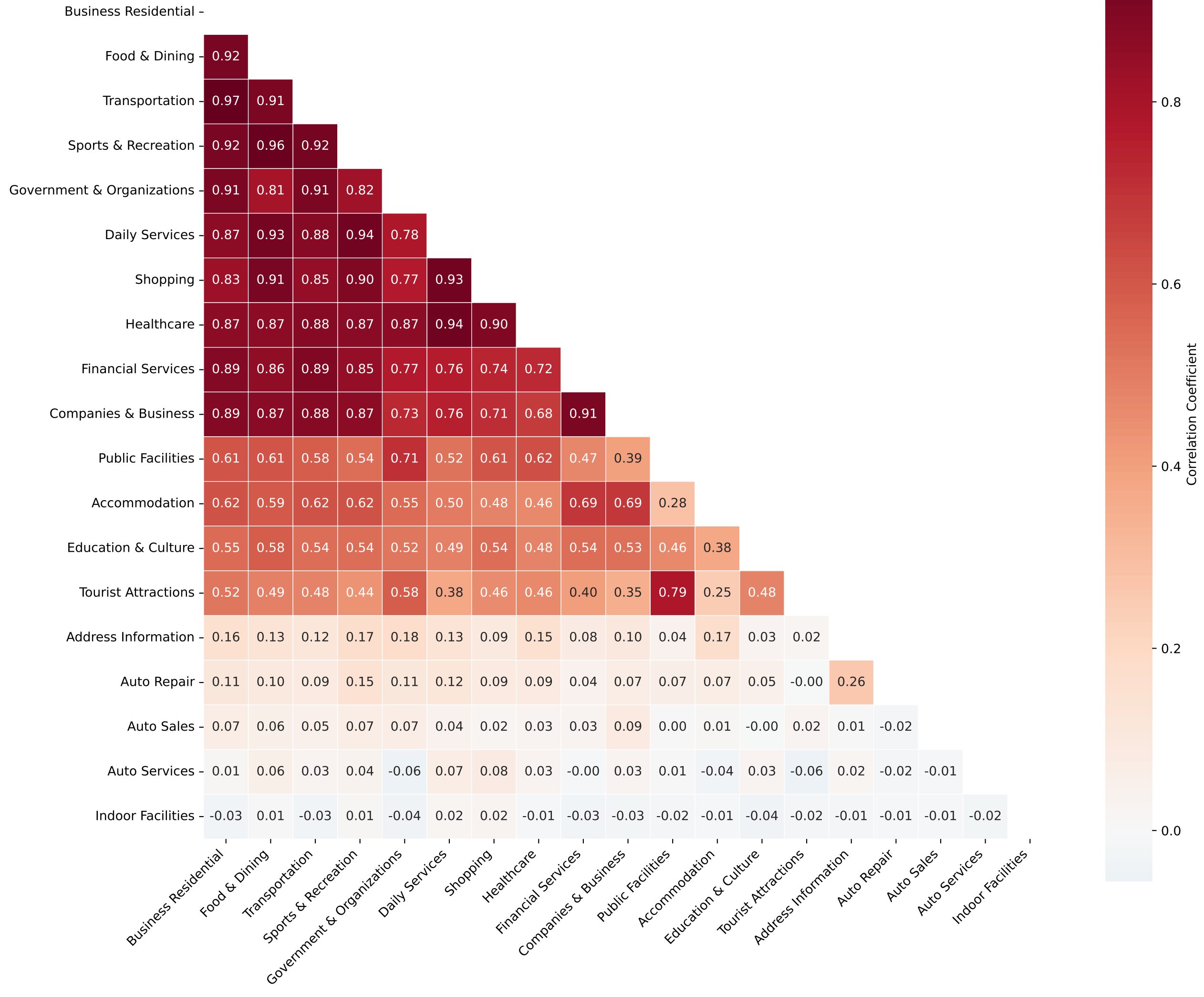
POI Category Correlation Matrix (Sorted by Correlation Strength)
