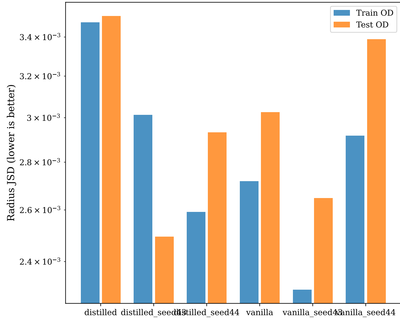
Radius of Gyration Distribution Quality
