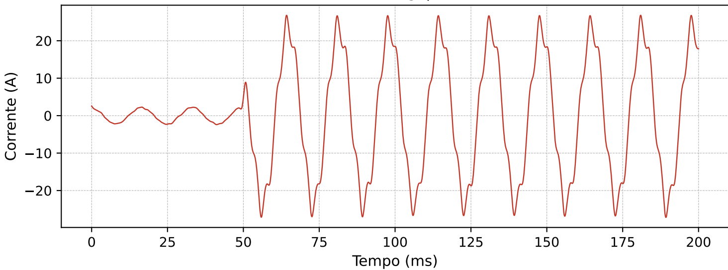
Sinal Filtrado — Hamming | RMSE = 0.70227
