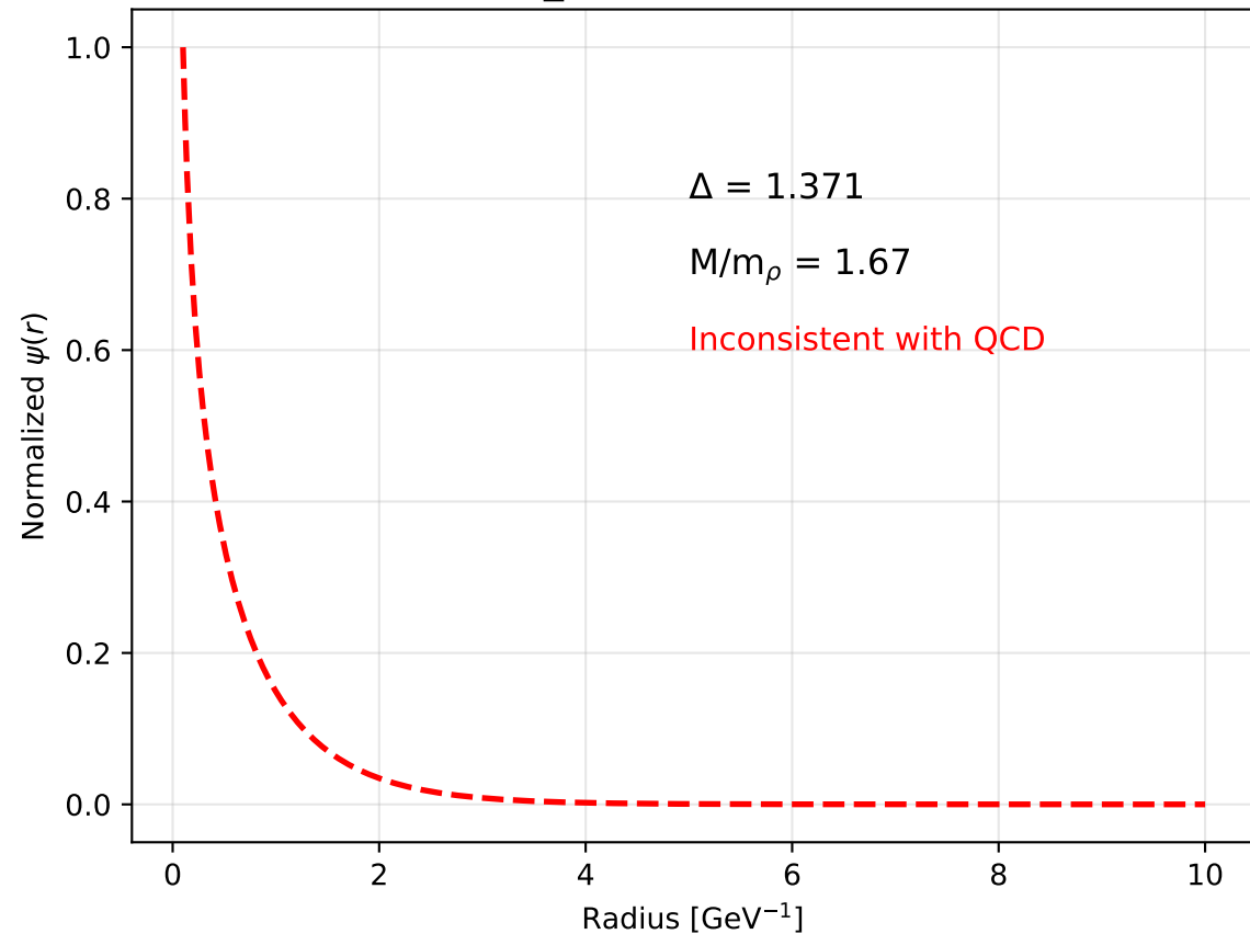
AdS_5: M = 1.29 GeV
