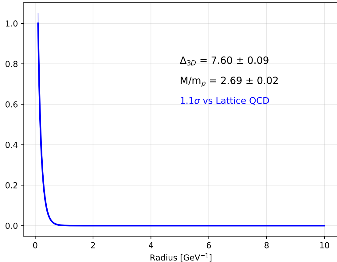
3D Physical: M = 2.08 ± 0.02 GeV
