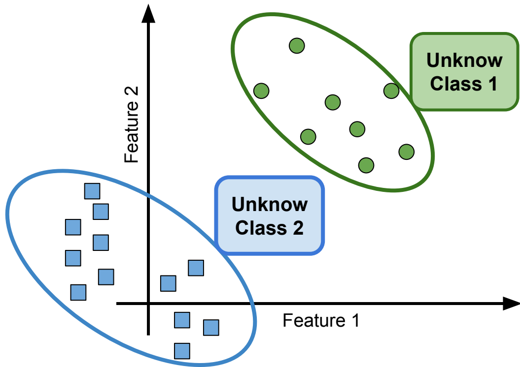
After K-Means
