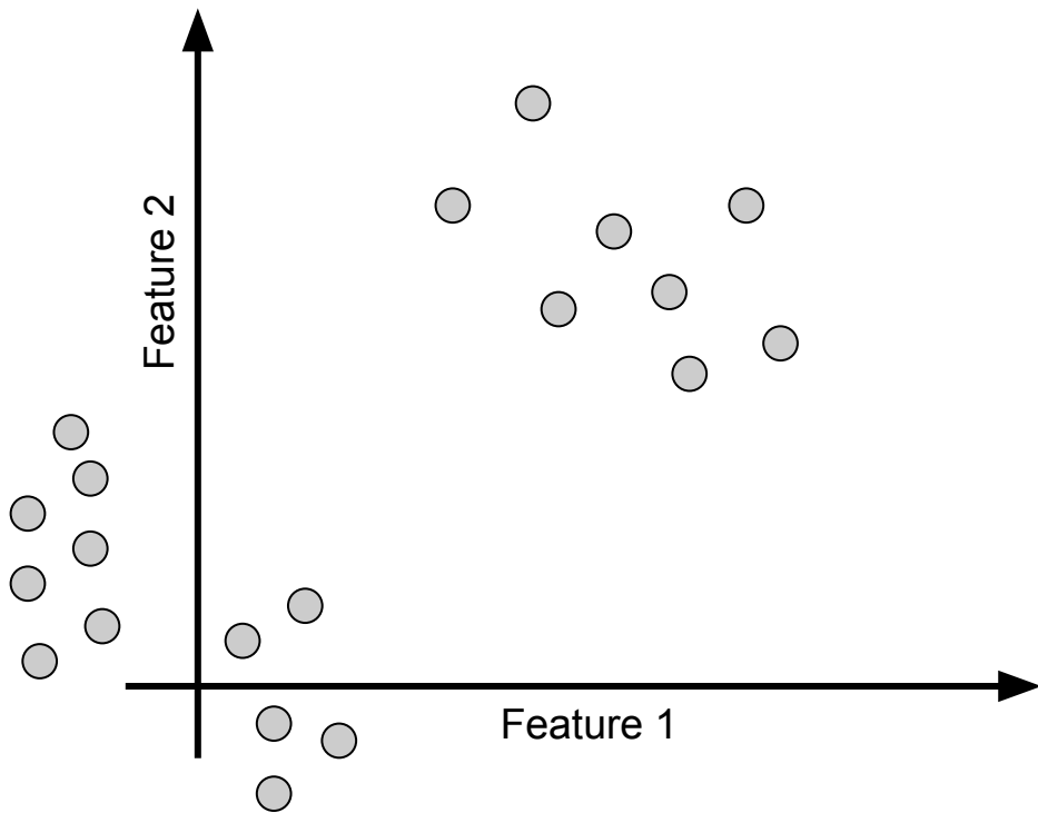
Before K-Means
