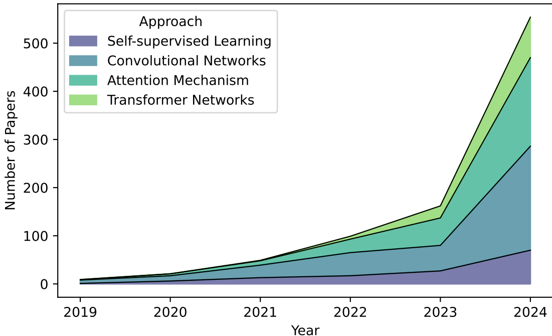
Cumulative Use of Transformers Over the Years
