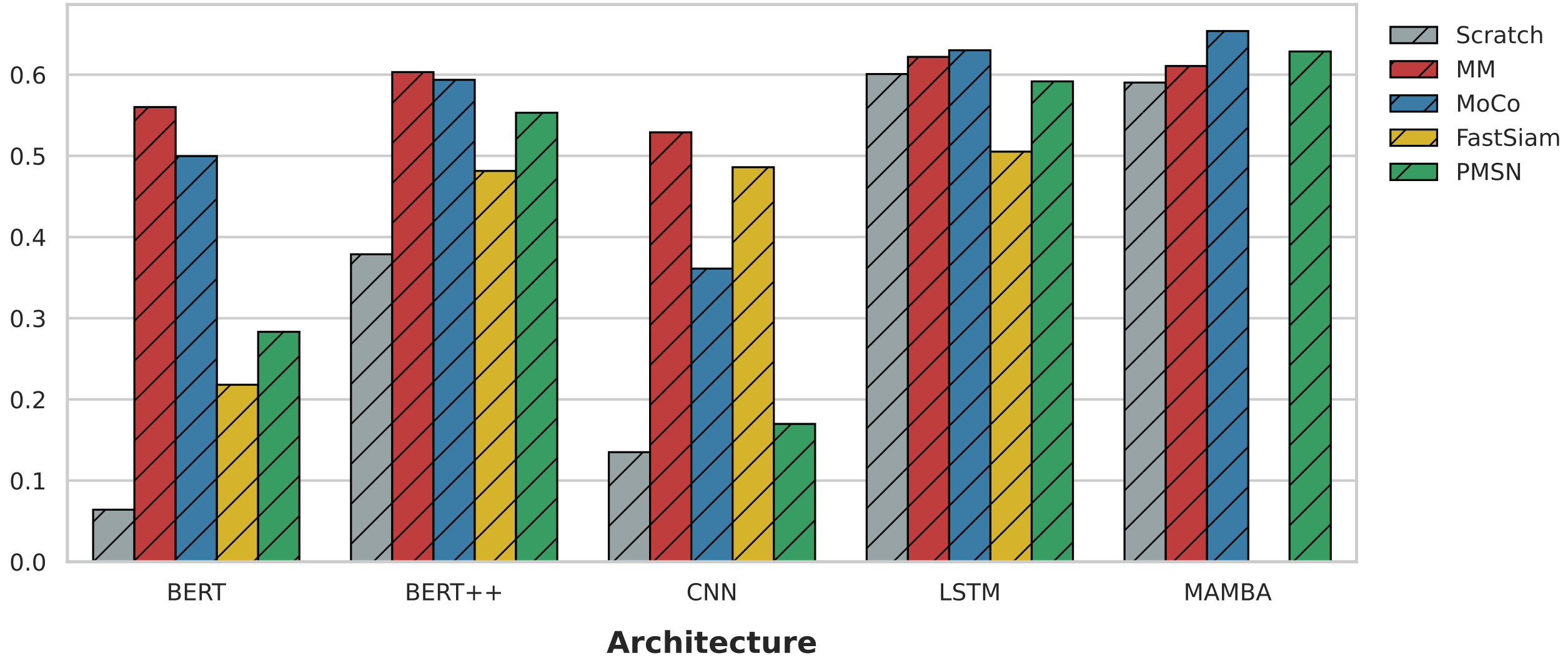
F1-Score (Weighted)
